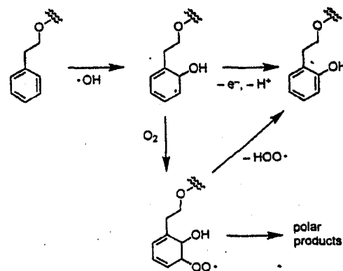
Fig. 3. Examples of typical reactions after addition of \cdot\text{OH} to the aromatic ring of phenethyl polyacrylate.
