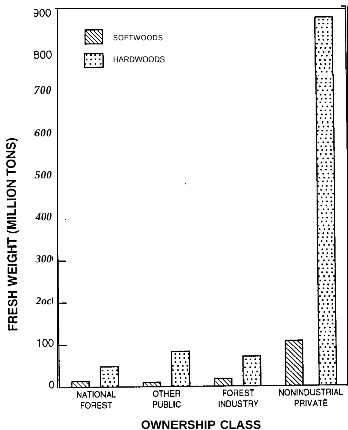
Figure 4.—Wood and bark, fresh, live-tree biomass for softwoods and hardwoods, by ownership class, Tennessee, 1989.
