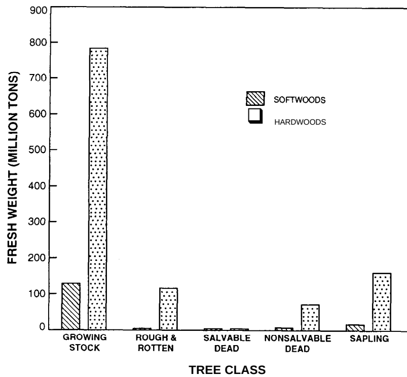
Figure 7.—Wood and bark, fresh, live-tree biomass for softwoods and hardwoods, by tree class, Tennessee, 1989.
