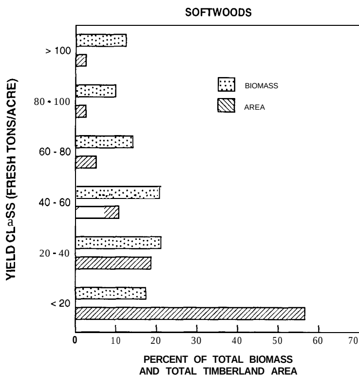
Figure 2.-Effective density of fresh, live-tree softwood biomass and relative area of softwood timberland by respective yield class, Tennessee, 1989.
