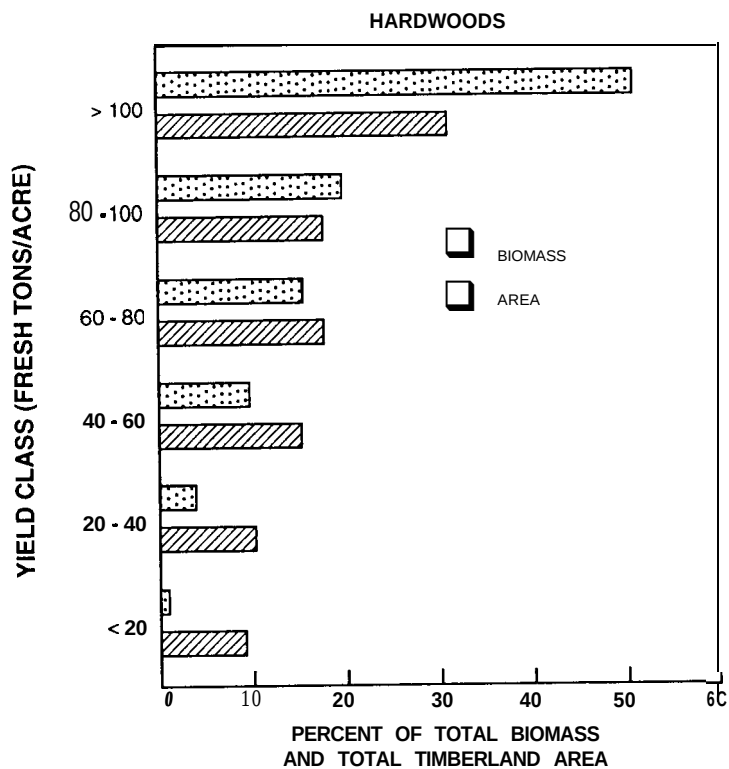
Figure 3.—Effective density of fresh, live-tree hardwood biomass and relative area of hardwood timberland by respective yield class, Tennessee, 1989.
