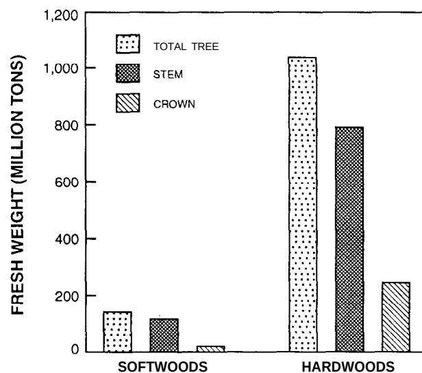
Figure 1.-Wood and bark, fresh, live-tree biomass for softwoods and hardwoods, by tree component, Tennessee, 1989.
