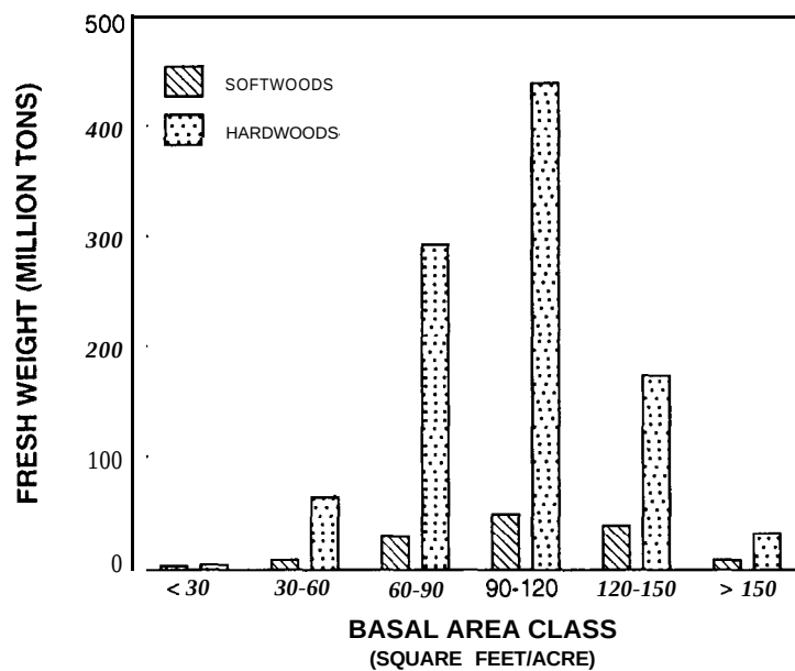
Figure 8.—Wood and bark, fresh, live-tree biomass for softwoods and hardwoods, by basal area class, Tennessee, 1989.
