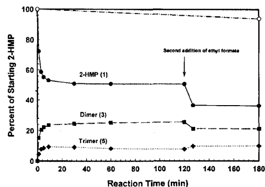
Figure 5 Reaction profile for self-condensation of 2-HMP (1) at 20 °C with added ethyl formate (filled symbols). Disappearance of 2-HMP at 20 °C without added ethyl formate (open symbols) is shown for comparison.
