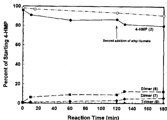
Figure 6 Reaction profile for self-condensation of 2-HMP (1) at 20 °C with added propylene carbonate.
