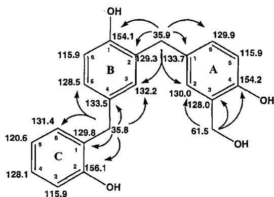
Figure 8 Assignment of experimental ^{13}\text{C} NMR data to proposed structure of trimer 5 isolated from self-condensation reaction of 2-HMP (1). Chemical shifts (ppm) for each carbon are indicated. Cross peaks in ^1\text{H} - ^{13}\text{C} long-range NMR correlation spectra were observed between hydrogen atom(s) on the carbon atom at which the arrows originate (hydrogen atoms not shown) and carbon atoms at the ends of the arrows.
