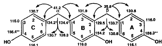
Figure 11 Assignment of experimental ^{13}\text{C} NMR data to proposed structure of trimer 8 isolated from self-condensation reaction of 4-HMP (2). Chemical shifts (ppm) for each carbon are indicated. Cross peaks in ^1\text{H} - ^{13}\text{C} long-range NMR correlation spectra were observed between hydrogen atom(s) on the carbon atom at which the arrows originate (hydrogen atoms not shown) and carbon atoms at the ends of the arrows.
