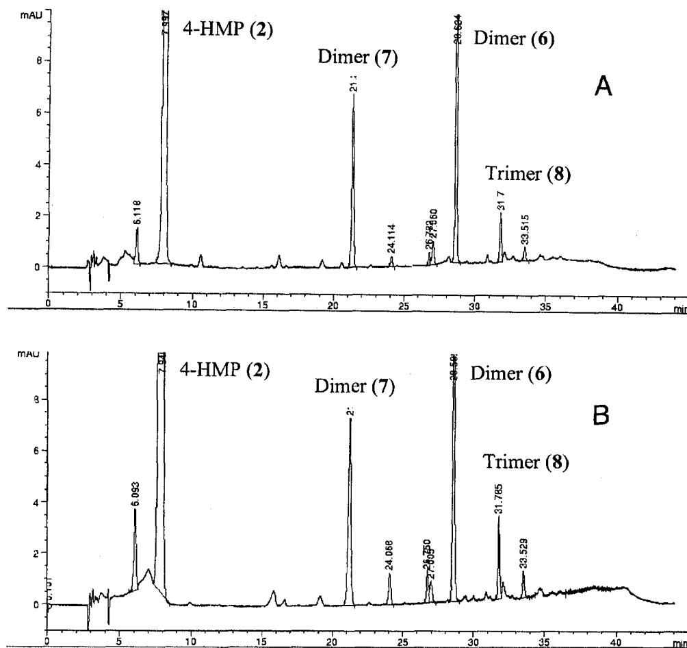
Figure 9 Comparison of (a) 4-HMP reacted at 20 °C with added ethyl formate as cure accelerator and (b) 4-HMP reacted at 60 °C without added cure accelerator by HPLC.
