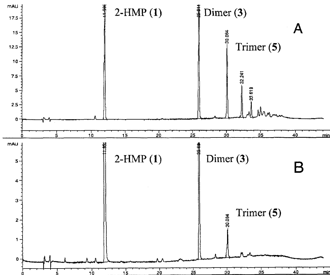
Figure 7 Comparison of (a) 2-HMP reacted at 20 °C with added propylene carbonate as cure accelerator and (b) 2-HMP reacted at 60 °C without added cure accelerator by HPLC.
