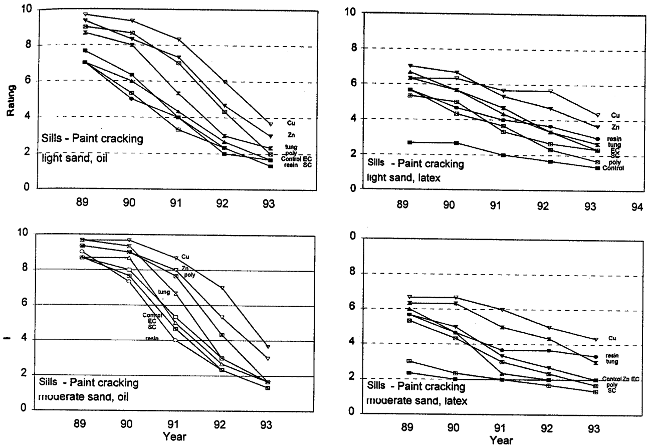
Figure 6. Mean ratings for cracking of windowsill paint after 5 years of outdoor exposure (10 means no observable degradation, and 1 means complete failure of the unit). All sills prepared with oil-alkyd primer. Oil designates oil topcoat; latex , acrylic-latex topcoat (Zn, zinc naphthenate WRP; EC, epoxide consolidant; resin, acrylic resin consolidant; Cu, copper naphthenate; SC, solvent-borne consolidant; tung, tung oil; poly, polyurethane varnish).
