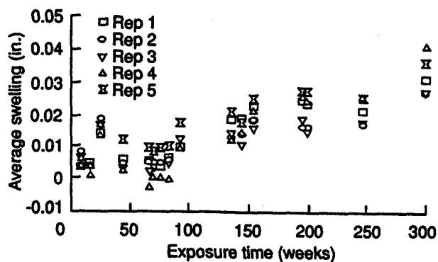
Figure 4. Average swelling of five replicate windows treated with WRP Treatment 7. Each data point is an average of two measurements. The shrinkage during dry periods is not shown (1 in. = 25.4 mm).
