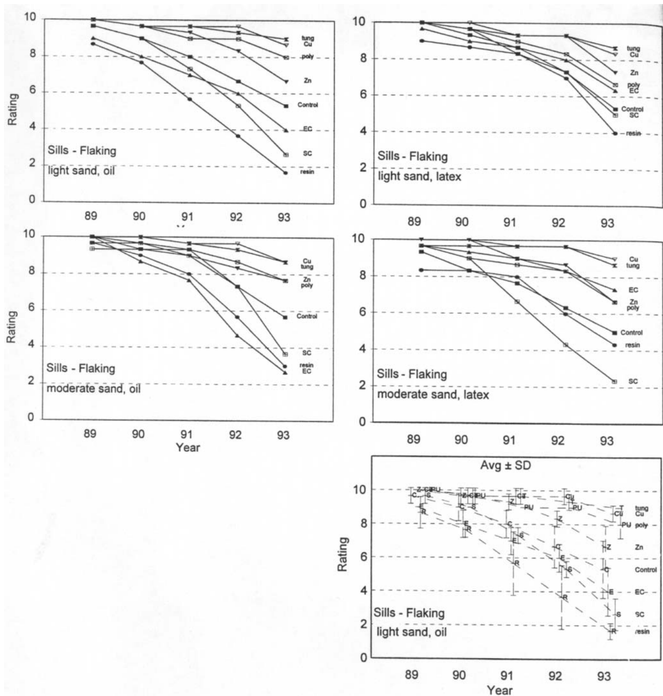
Figure 5. Mean ratings for flaking of windowsill paint after 5 years of outdoor exposure (10 means no observable degradation, and 1 means complete failure of the unit). All sills were prepared with oil-alkyd primer. Oil designates oil topcoat; latex , acrylic-latex topcoat. Lower right graph shows distribution of ratings for each pretreatment (Zn, zinc naphthenate WRP; EC, epoxide consolidant; resin, acrylic resin consolidant; Cu, copper naphthenate; SC, solvent-borne consolidant; tung, tung oil; poly, polyurethane varnish).
