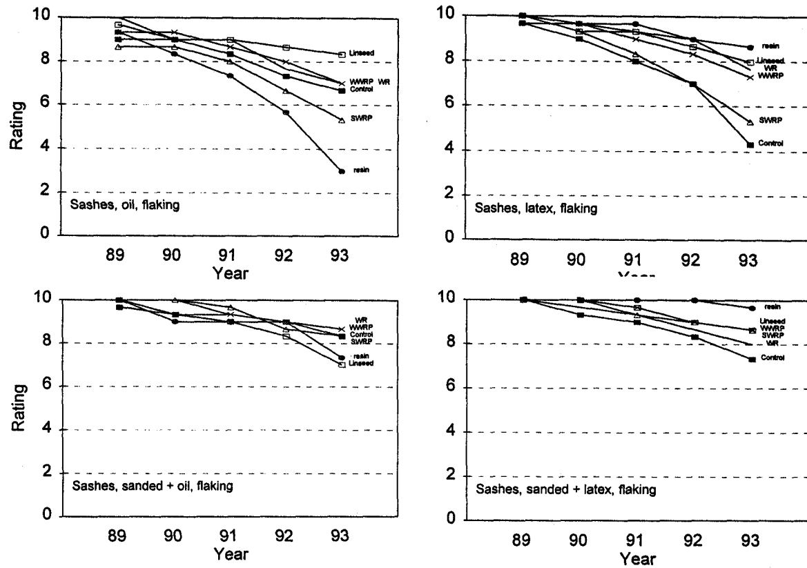
Figure 7. Mean ratings for flaking of window sash paint after 5 years of outdoor exposure (10 means no observable degradation, and 1 means complete failure of the unit). Oil designates oil-alkyd primer and topcoat; latex , acrylic-latex primer and topcoat (SWRP, solvent-borne WRP; WR, water repellent; Linseed, linseed oil; WWRP, waterborne WRP; resin, acrylic resin).
