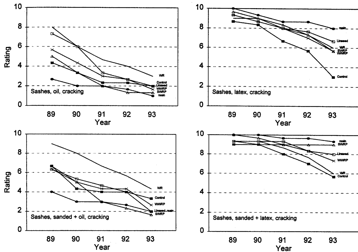
Figure 8. Mean ratings for cracking of window sash paint after 5 years of outdoor exposure (10 means no observable degradation, and 1 means complete failure of the unit). Oil designates oil-alkyd primer and topcoat; latex , acrylic-latex primer and topcoat (SWRP, solvent-borne WRP; WR, water repellent; Linseed, linseed oil; WWRP, waterborne WRP; resin, acrylic resin).
