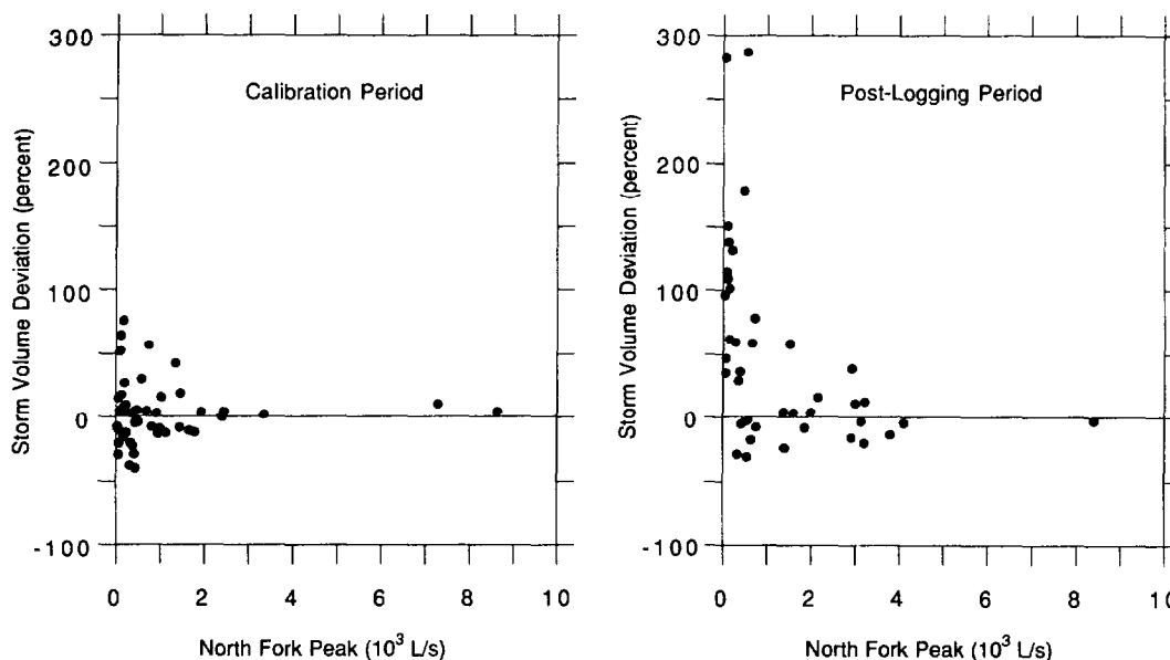
Fig. 7. Deviation of observed South Fork storm volumes from predicted volumes during the calibration and logged periods as a function of peak flow in the North Fork.
