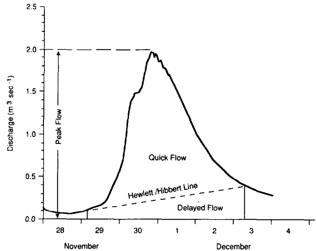
Fig. 2. Hydrograph separation applied to runoff from the North Fork of Caspar Creek between November 29, 1973, and December 3, 1973 (adapted from Krygier and Harr [1972]).
