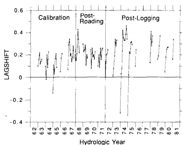
Fig. 6. LAGSHIFT (the relative change in the South Fork lag time) within each hydrologic year during the study.
