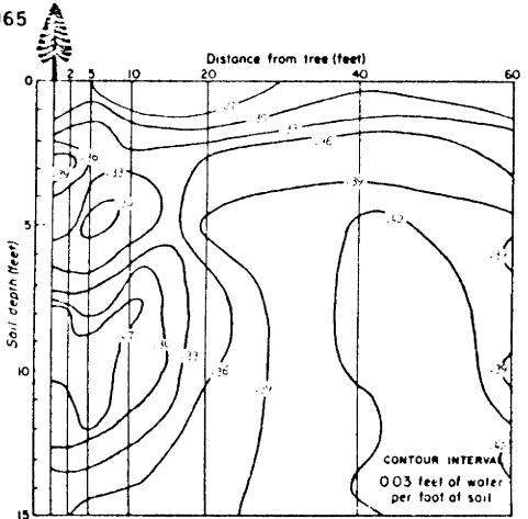
Figure 12. Isopleths of soil moisture in the partially cut study plot I.1 on a) August 16, b) September 14, and c) October 19, 1965.
