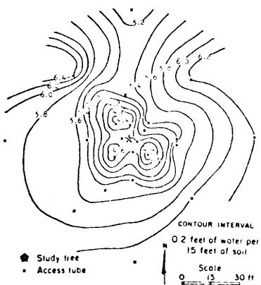
Figure 12. Isopleths of soil moisture in the partially cut study plot I.1 on a) August 16, b) September 14, and c) October 19, 1965.
