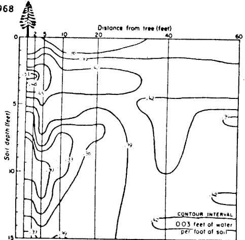
Figure 23. Isopleths of soil moisture in the isolated tree study plot L1 on a) September 25, b) October 9, and c) October 23, 1968.
