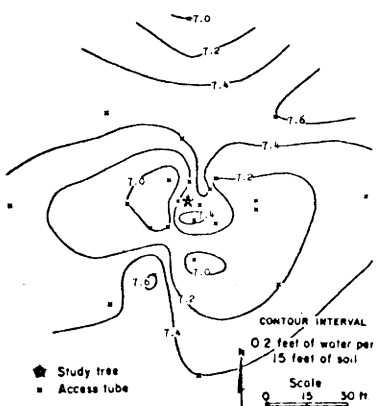
Figure 13. Isopleths of soil moisture in the partially cut study plot L1 on a) November 30, 1965, b) January 17, and c) February 11, 1966.
