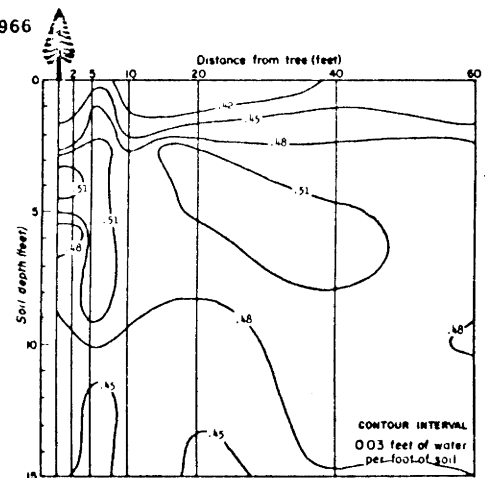
Figure 13. Isopleths of soil moisture in the partially cut study plot L1 on a) November 30, 1965, b) January 17, and c) February 11, 1966.
