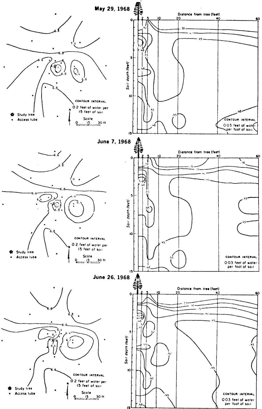
Figure 21. Isopleths of soil moisture in the isolated tree study plot L1 on a) May 29, b) June 7, and c) June 26, 1968.
