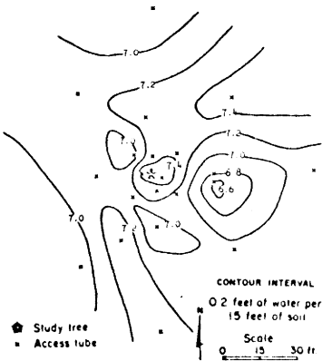
Figure 24. Isopleths of soil moisture in the isolated tree study plot L1 on a) January 7, 1969 and in the bare study plot L1 on b) March 27, and c) May 5, 1969.
