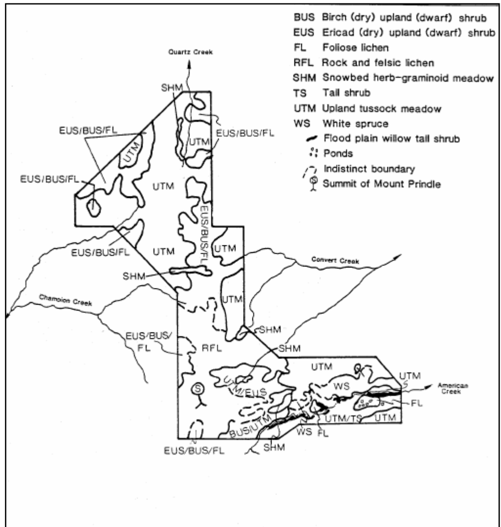
Figure 16—Vegetation cover map of Mount Prindle Research Natural Area; interpreted from NASA color infrared high altitude aerial photo at approximate contact scale of 1 :63,000, project 02929 ALK 60, frame number 8863, photo taken August 5, 1980.
