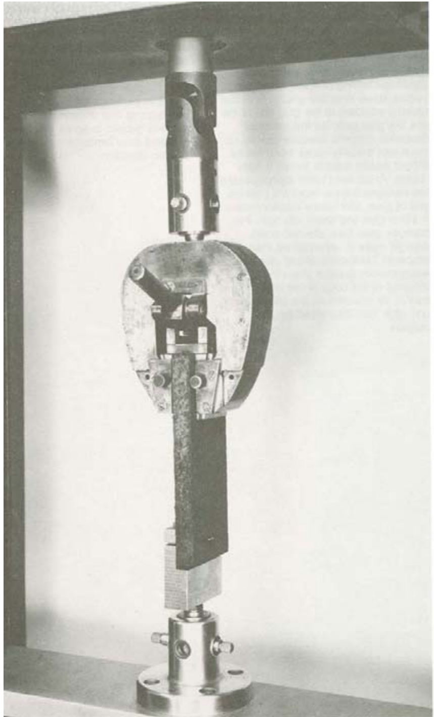
Figure 12.—Test setup for measuring lateral staple resistance of fiberboards. Lewis 1962a. (M121 368)
