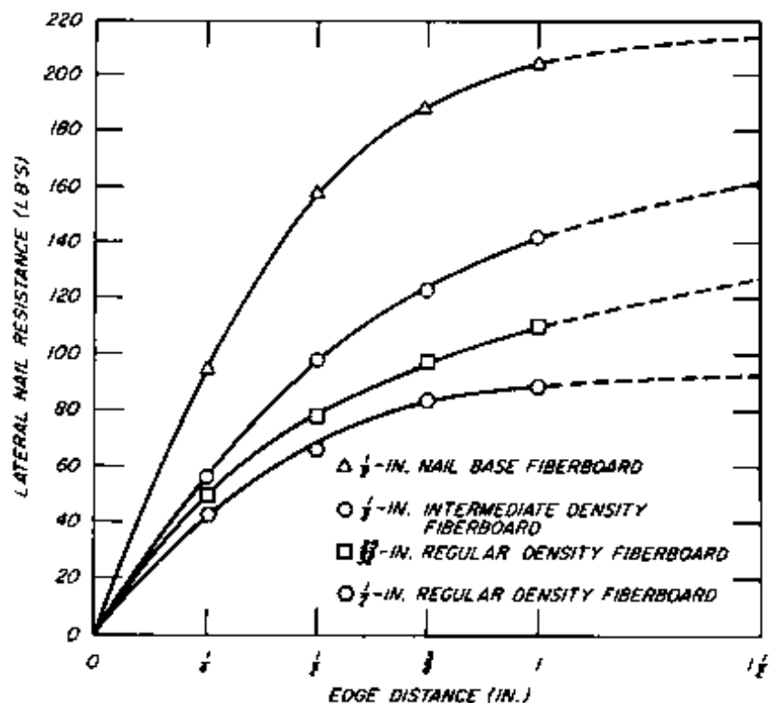
Figure 10.—Lateral nail resistance at various edge distances for four types of cellulosic fiberboard. Tuomi and Gromala 1977. (M144 300)
