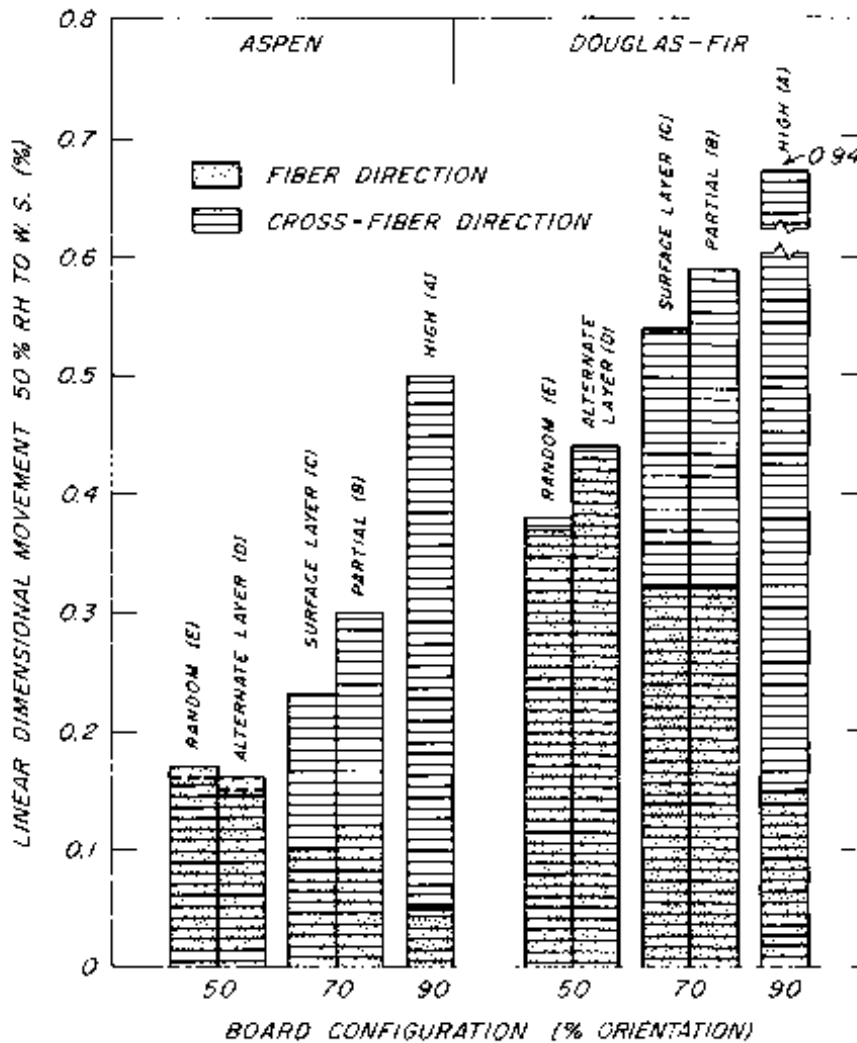
Figure 3.—Relationship of linear dimensional movement to quantity and location of oriented fibers of aspen and Douglas-fir high-density hardboards. (See Fig. 2 legend for Key, A-E.) Steinmetz and Polley 1974. (M141 026)
