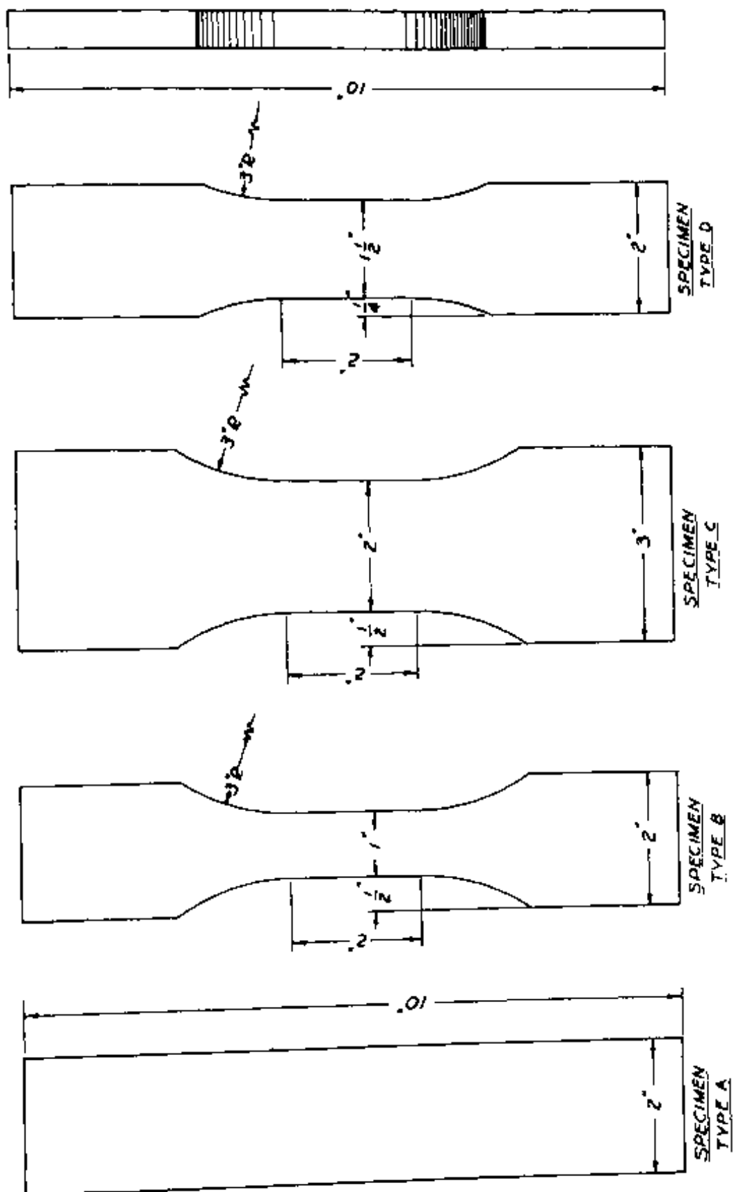
Figure 15.—Details of tension parallel-to-surface specimens for comparative tests on cellulosic fiberboard. Lewis 1948. (ZM777 13F)
