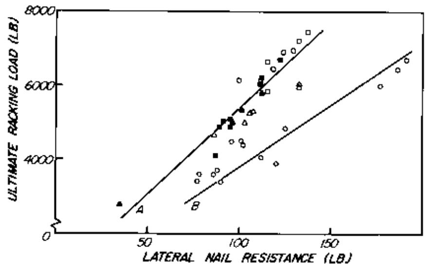
Figure 9.—Relationship between lateral nail resistance of fiberboard sheathing and racking resistance of walls sheathed with fiberboard. (ML85 5063). The equation for line A is from Neisel and Guerrero (1956), with data points from Luxford (1957a) (Dry \Delta , Wet \blacktriangle ) and Neisel and Guerrero (1956) (Dry \square , Wet \blacksquare ). Equation and data points (Dry \circ ) for line B are from Tuomi and Gromala (1977).
