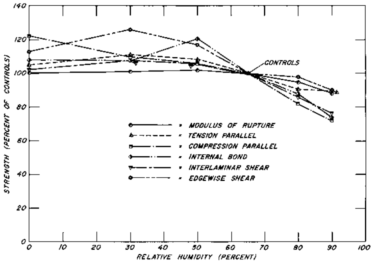
Figure 17.—Average strength of six 1/4-inch-thick tempered hardboards oven-dried and conditioned to equilibrium moisture content at five relative humidities. McNatt 1974. (M141 011)
