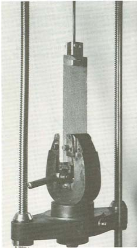
Figure 8—Test setup for measuring lateral nail resistance of fiberboard according to ASTM Standard D 1037. (M766 00)
