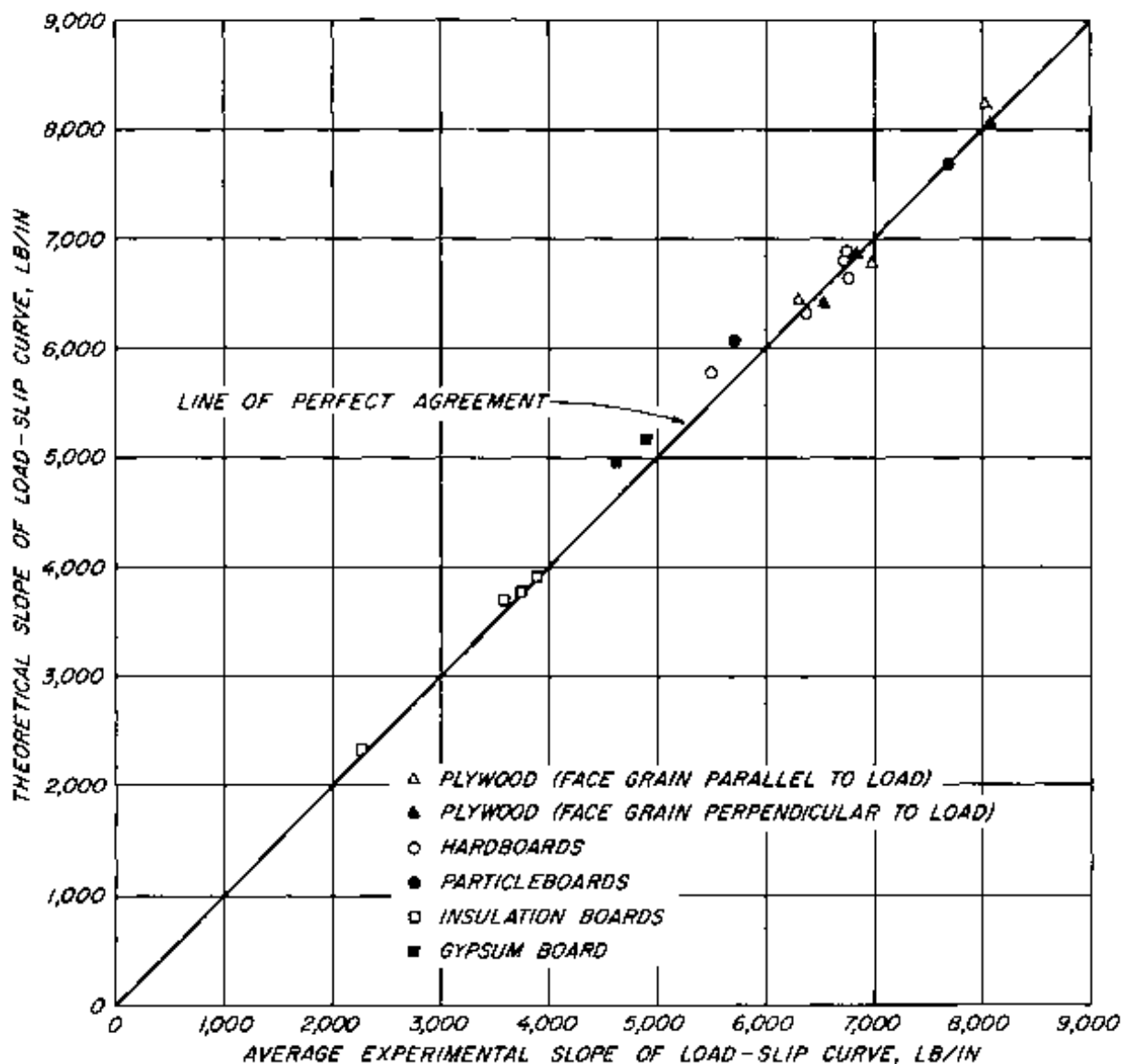
Figure 11.—Theoretical versus experimental slopes of the load-slip curve for joints with one member of Douglas-fir lumber and one member of panel material. Wilkinson 1972. (M141 657)
