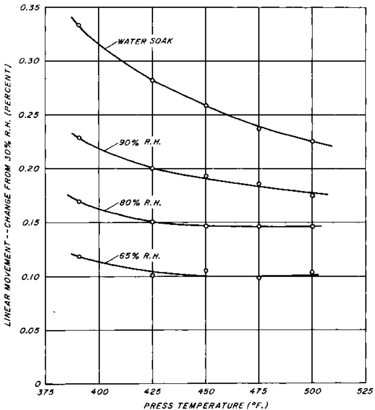
Figure 4. —Relationship between linear movement and hot pressing temperature for 1/8-inch-thick high-density hardboards. Steinmetz 1970. (M137666)
