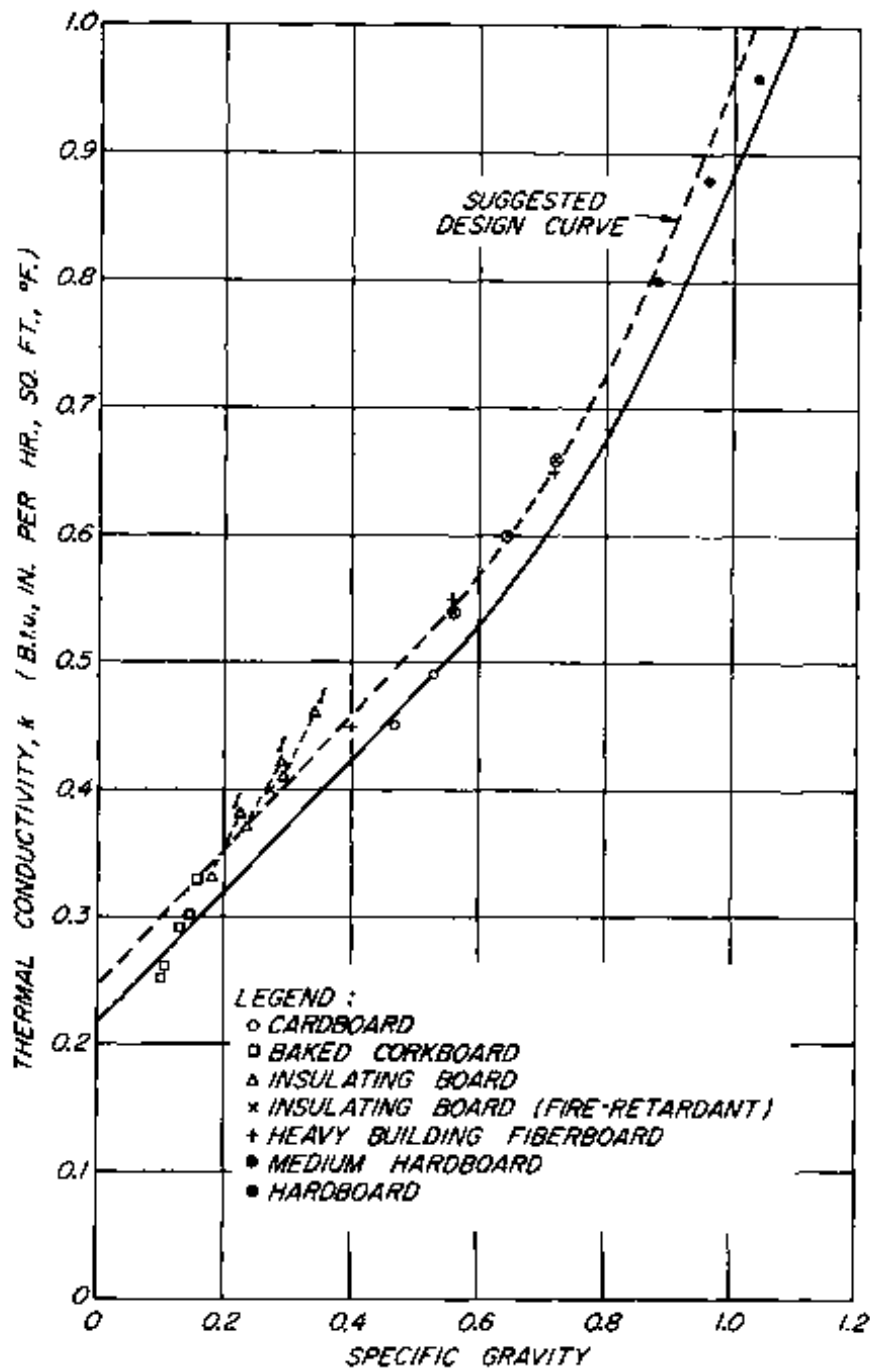
Figure 6.—Relationship between thermal conductivity and specific gravity for wood-base fiber materials and suggested design curve. Lewis 1967. (M132 875)
