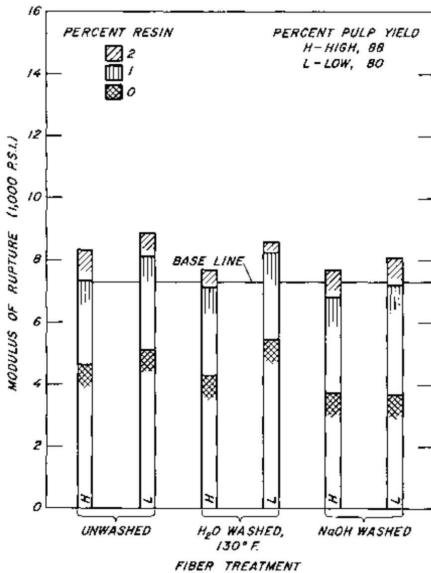
Figure 1.—Relationship of modulus of rupture to fiber treatment of wet-formed red oak hardboards. Steinmetz 1973. (M141 229)
