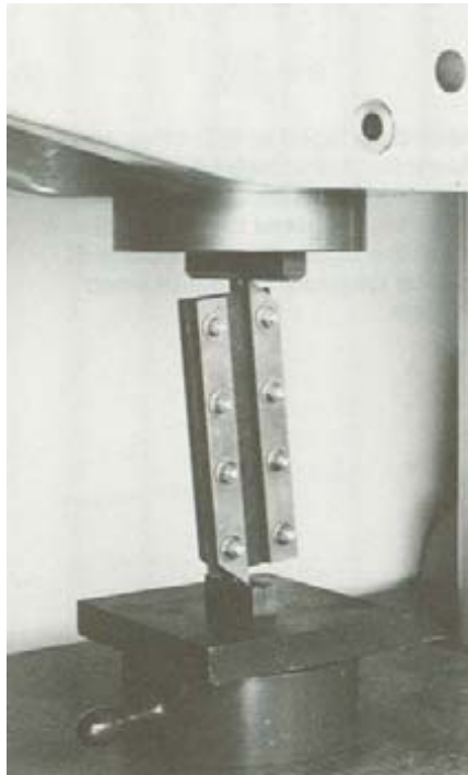
Figure 13.—Rail shear test setup for measuring edgewise shear strength of hardboard. ASTM Standard D 1037. (M125 798)
