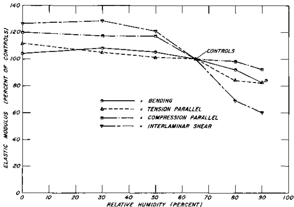
Figure 16.—Average elastic moduli of six 1/4-inch-thick tempered hardboards ovendried and conditioned to equilibrium moisture content at five relative humidities. McNatt 1974. (M141 014)
