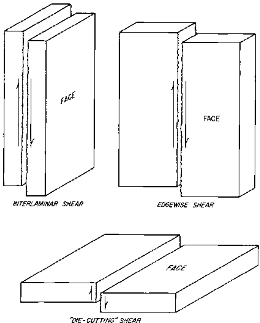
Figure 14.—Three basic shearing directions for hardboard (character of failure not necessarily as shown). McNatt 1972. (M139 209)
