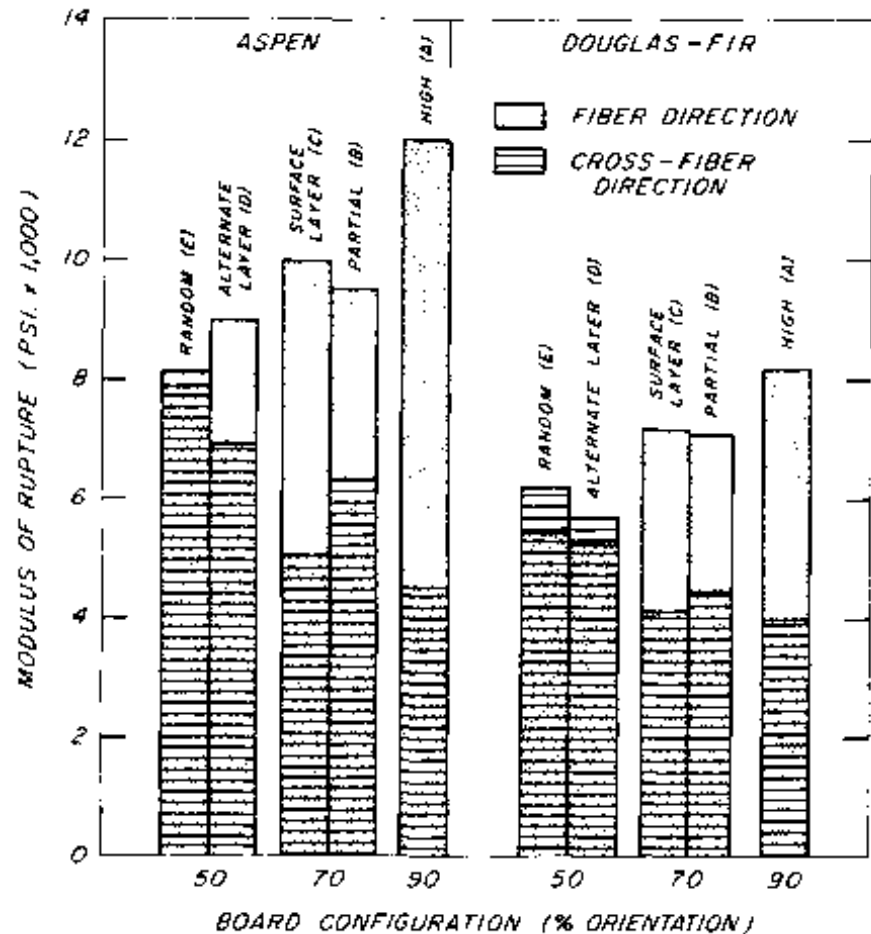
Figure 2.—Relationship of modulus of rupture to quantify and location of oriented fibers of aspen and Douglas-fir high-density hardboards. (A, highly oriented; B, partially oriented—one-half of fibers by weight were oriented; C, partially oriented, oriented fibers concentrated on surface layers, randomly oriented in center half; D, alternate layers oriented, fibers in adjacent layers perpendicular to preceding layer; and E, randomly oriented control board.) Steinmetz and Polley 1974. (M141 025)
