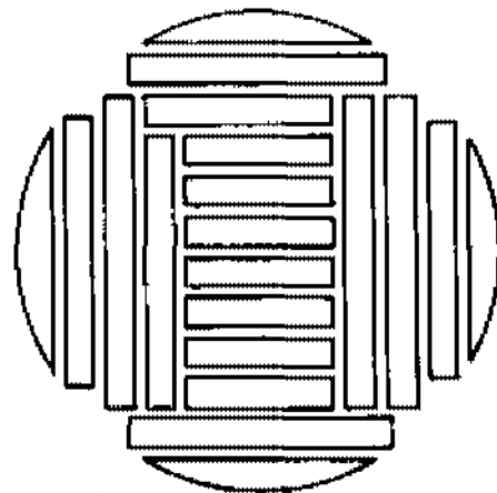
Figure 4.—End view of log "grade sawn: by the decision sawing method. (M 148 325)
