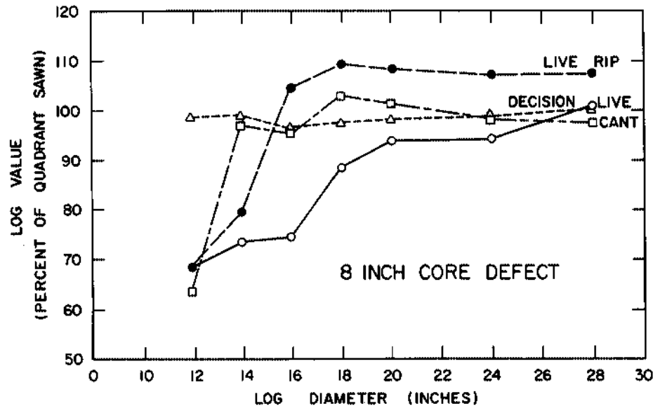
Figure 11.—Lumber values for four sawing methods as percentages of values from quadrant-sawn logs with an 8-inch-diameter core defect.
