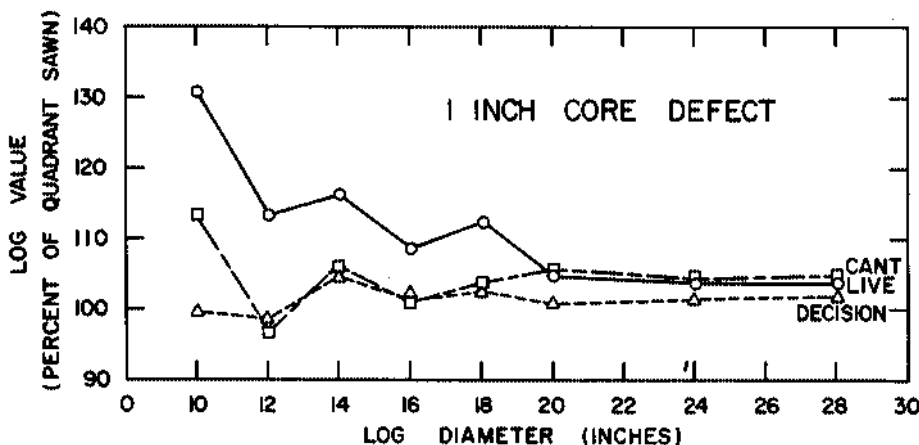
Figure 8.—Lumber values for three sawing methods, as percentages of values from quadrant-sawn logs with a 1-inc core defect.
