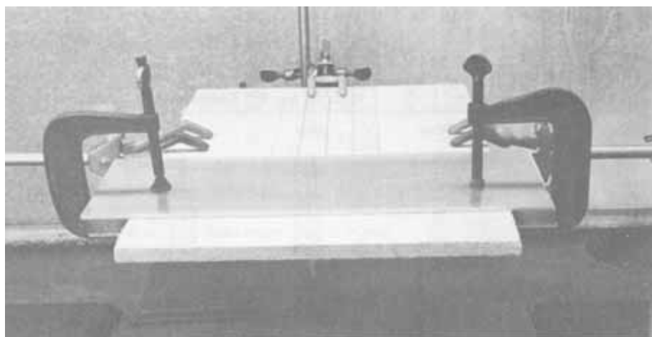
Figure 3.—Specimen with plates clamped in place just prior to ignition.
