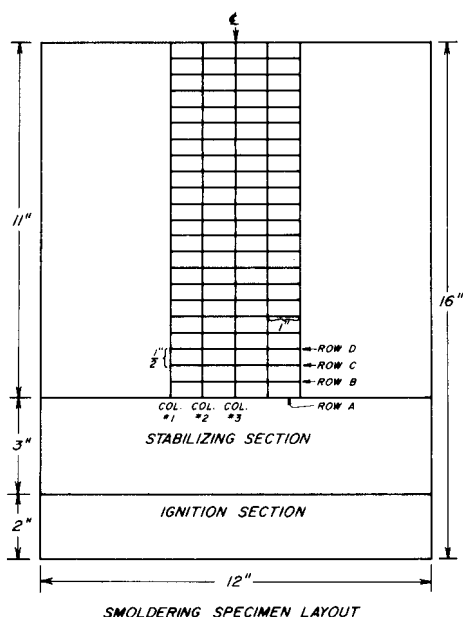
Figure 1.—Specimen with scribed grid for smoldering test.
