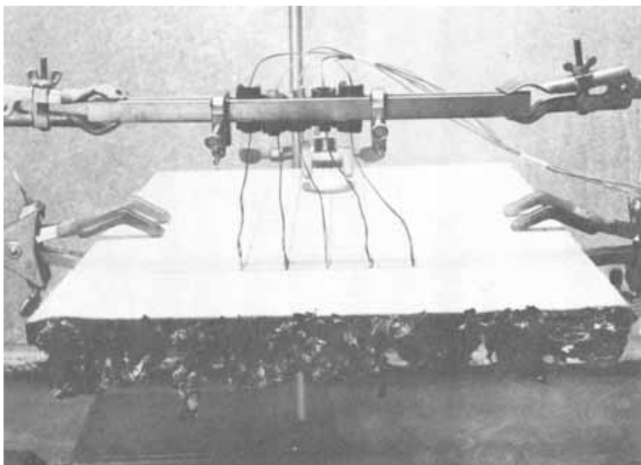
Figure 4.—Smoldering specimen with thermocouples in row A and circular level gage in front of rear clamp.
