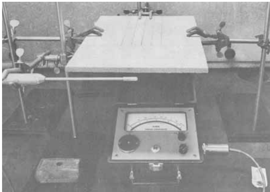
Figure P.—Level specimen with probe in place for approach-air velocity measurement.
