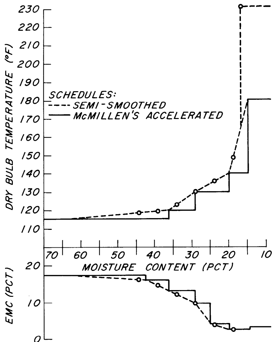
Figure 2.—Construction of smoothed-accelerated schedule for white oak.
