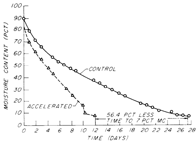
Figure 4.—Comparison of drying time of 4/4 northern red oak dried by conventional schedule and by accelerated techniques (presurfaced, presteamed, accelerated-smoothed schedule, high-temperature dried below 18 percent MC).
