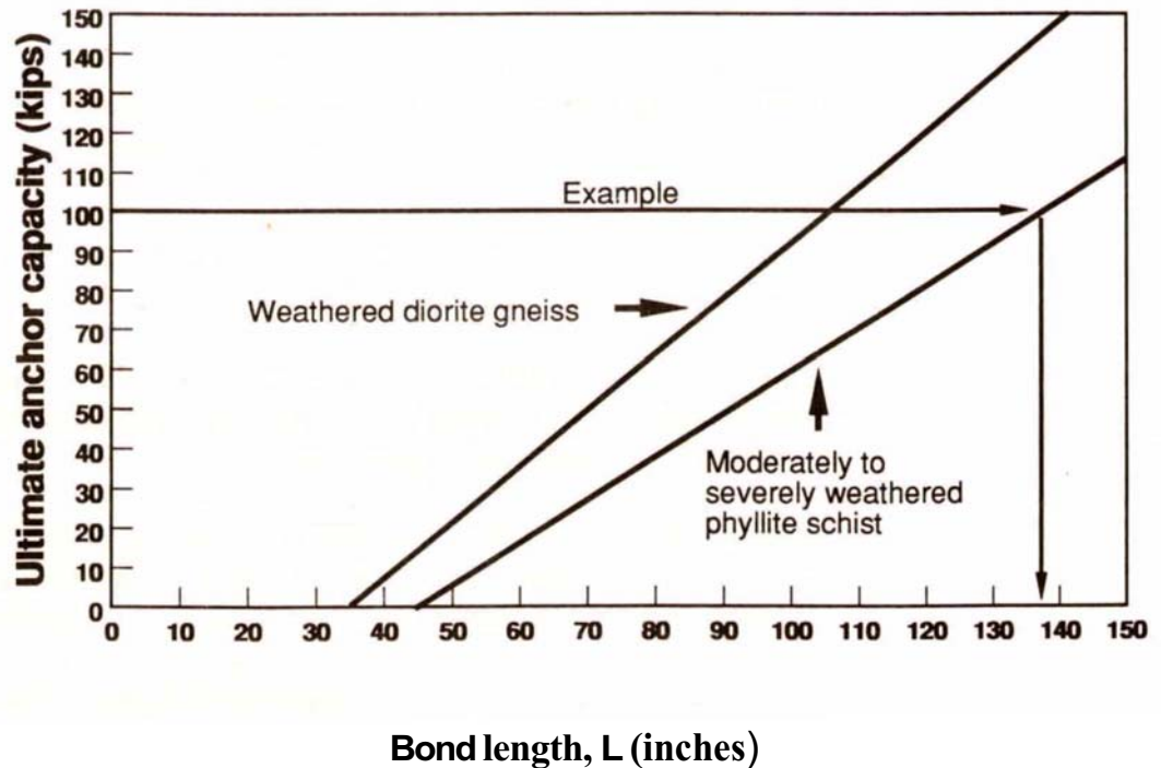
Figure 3. Ultimate anchor capacity as a function of grouted bond length in rock. This figure is based on results of anchor tests in rocks commonly found on Wrangell Island, southeast Alaska, and should be used with care at other localities where extensive weathering, fracturing, and discontinuous rock units are encountered.
