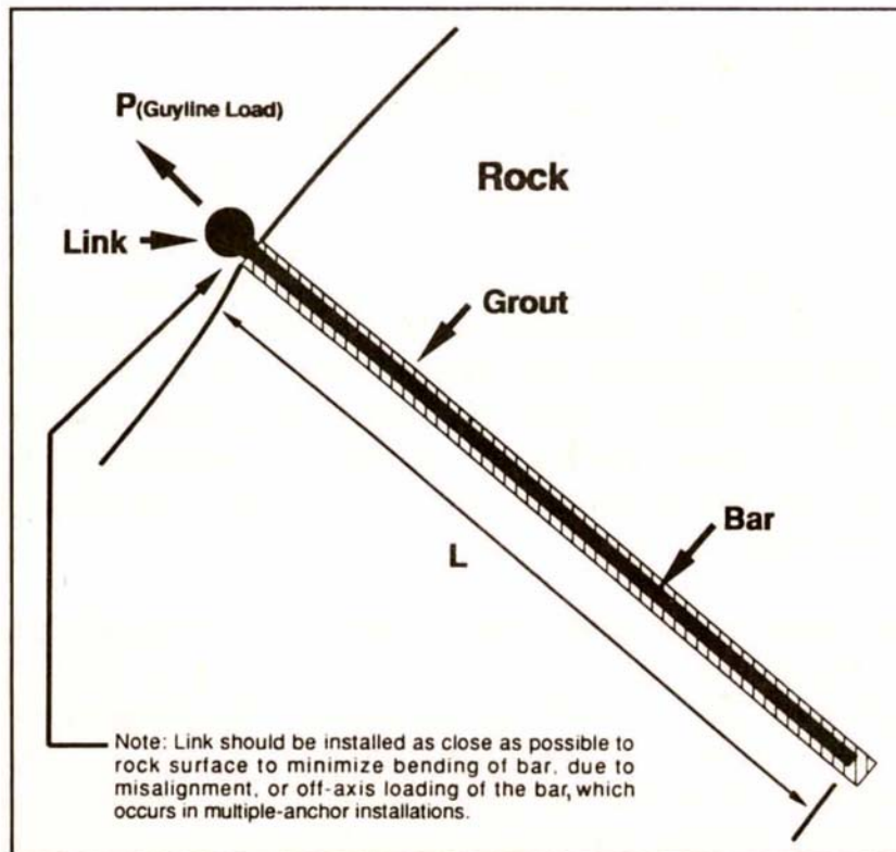
Figure 1-Elements of a grouted rock anchor P is total guyline force or 'load.' A 'link' is the mechanical connection between the guyline and the anchor. (One kip equals 1,000 pounds.)
