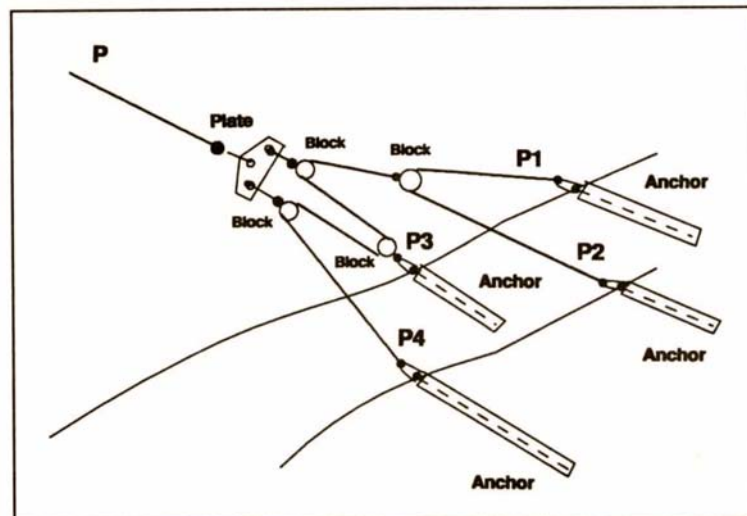
Figure 6-Example of a multiple anchor system for large guyline loads employing blocks to equalize line tensions. P is total guyline force. P1 - P4 are tether forces.
