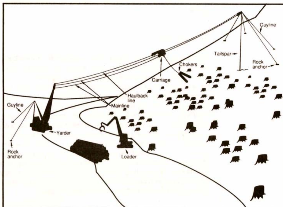
Figure 2- Typical rigging for skyline logging showing cable attachment locations where rock anchors can be effective .
