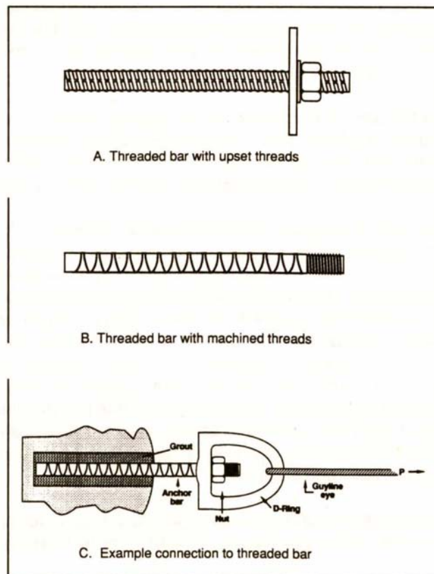
Figure 4—Examples of threaded bars used for anchors: (A) threaded bar with upset threads (Dywidag Systems International 1986); (B) threaded bar with machine threads (Williams Form Engineering Corp 1988); and (C) common D-ring connection or "link" between guyline and threaded bar.
