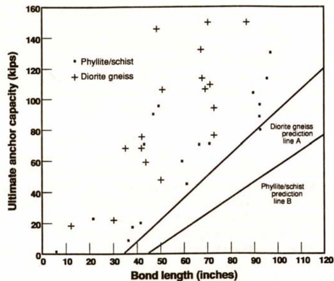
Figure 7-A plot of the ultimate anchor capacity versus bonded length for 34 test sites in phyllite/schist and diorite gneiss on Wrangell Island, southeast Alaska. Lines A and B were obtained by linear regression analysis and represent the lower 95-percent prediction limits for rock types tested. Anchor capacity is extrapolated above 110 kips.
