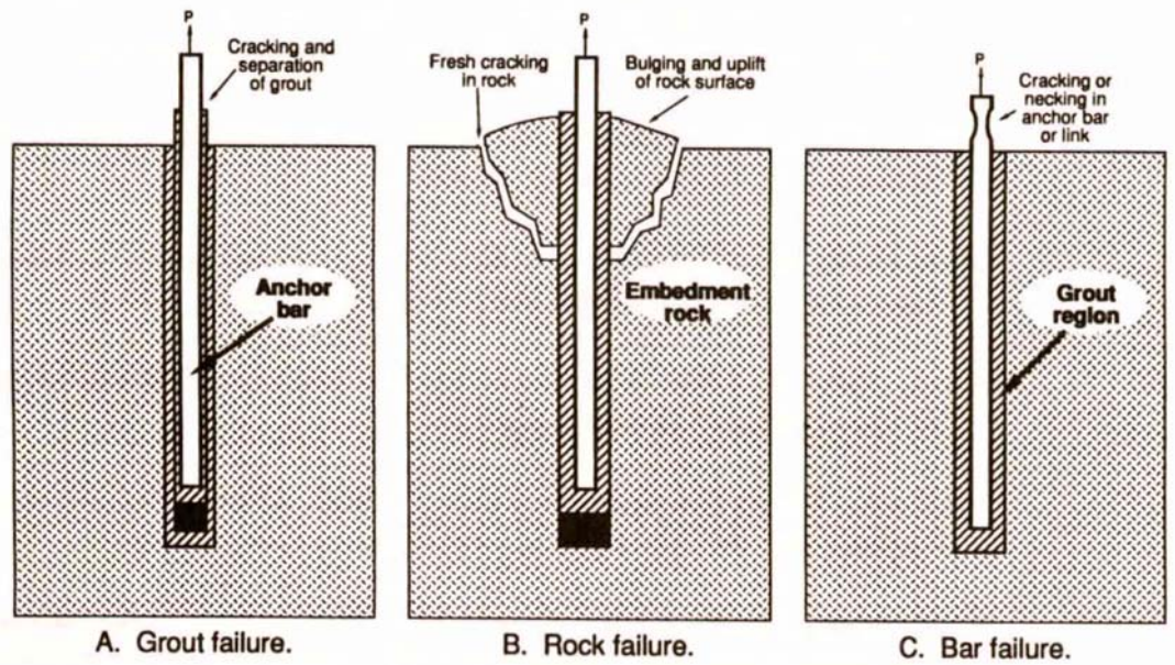
Figure 5_Three common failure modes for rock anchors: (A) failure of the grout; (B) failure of the rock mass; and (C) failure of the anchor bar.
