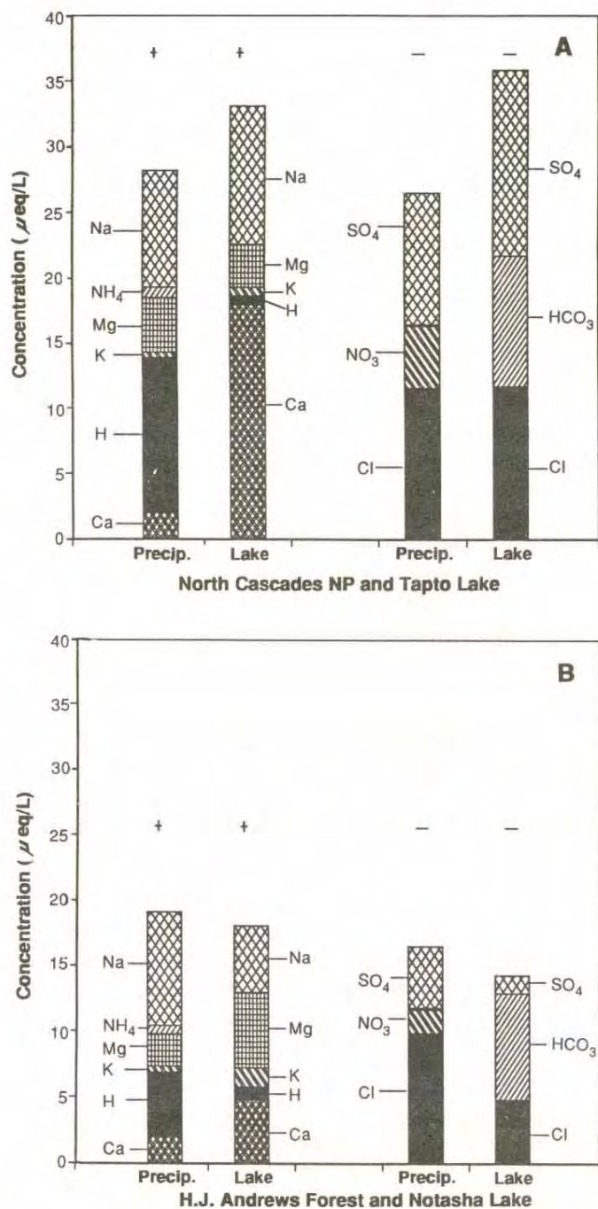
Figure 2—Major ion chemistry of precipitation at two NADP/NTN (1987) sites and adjacent dilute lakes sampled in the western lakes survey (Landers and other 1987) near the NADP sites. Both the precipitation and lake chemistry are from 1985. A: NADP/NTN site is at North Cascades National Park, WA (elevation 120 meters); lake sample is Tapto Lake, 4B1-051 (elevation 1744 meters). B: NADP/NTN site is H J Andrews Experimental Forest, OR (elevation 436 meters); lake sample is Lake Notasha, 4B1-060 (elevation 1836 meters).
