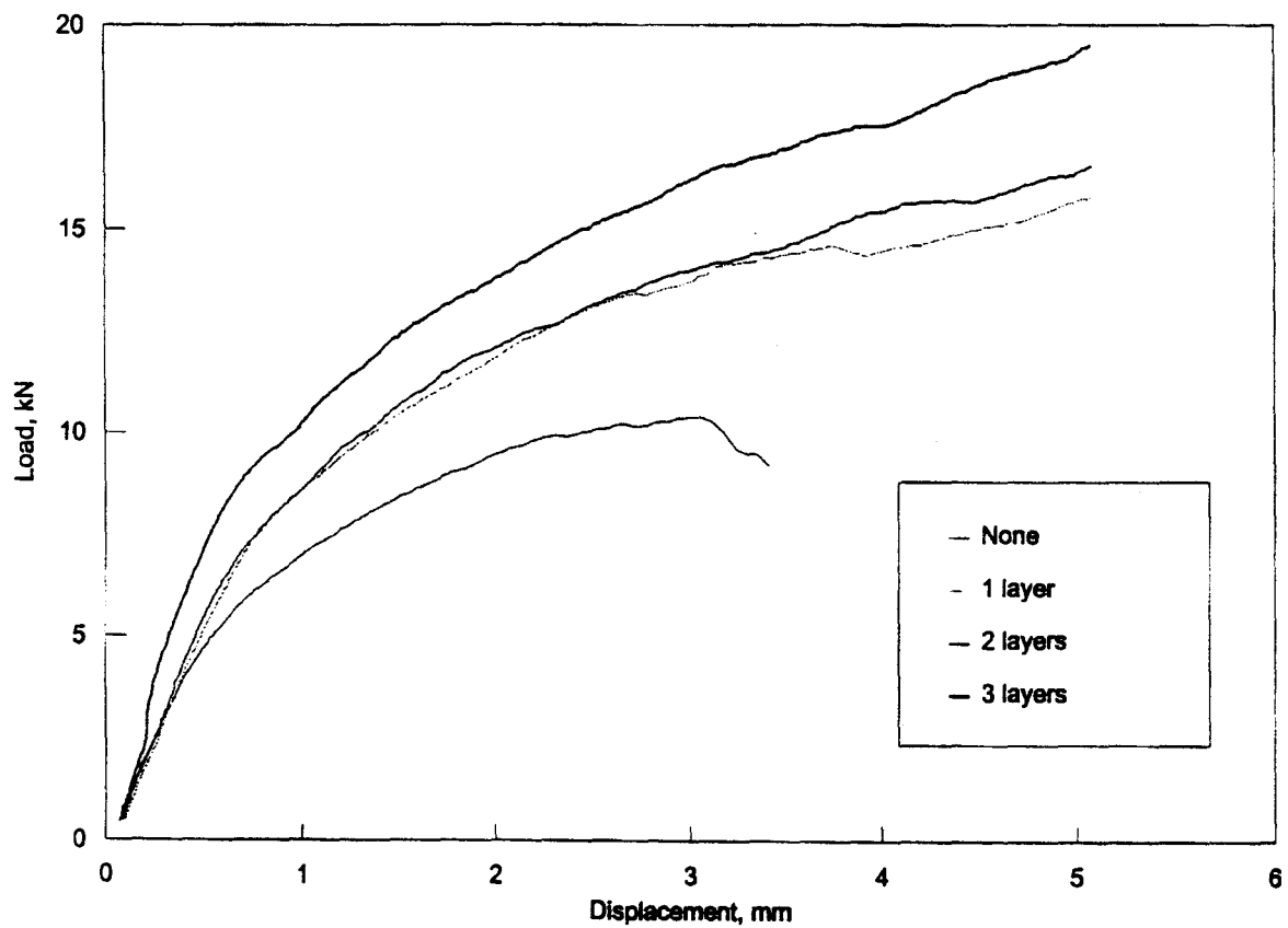
Figure 3.—Typical load versus displacement curve for fiberglass reinforced bolted connection loaded perpendicular-to-grain.
