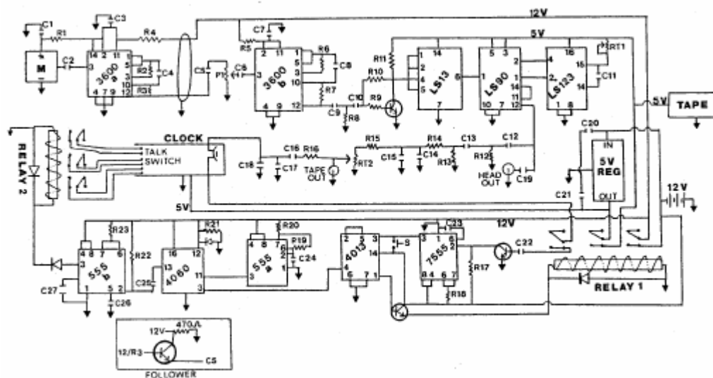
Figure 1—Circuit diagram for the automated bat detector system, based on Miller and Andersen (1984). See table 2 (in text) for a parts list. Integrated circuit connecting pins are indicated. Microphone, clock, and tape recorder specifications and sources are given in table 3 (in text). Inset shows the configuration of a following circuit to be added at pin 12/R3 if audio shielded cable >20m is used for the microphone cable. M=microphone; S=reset button; C=capacitor; R=resistor.
