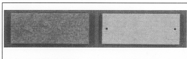
2. Left, polypropylene (unweathered) test specimens with 50% wood flour left; right, polypropylene (weathered) specimen (1500 hr.).
