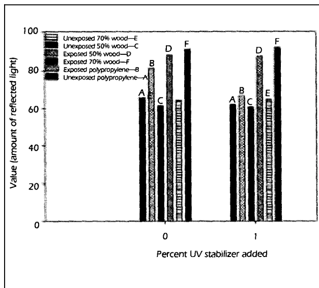
5. Effect of W stabilizer on color fade of wood flour polypropylene composites.
