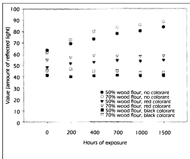
3. Effects of pigments and fiber content on color fade of HDPE wood flour composites (only colorant added).
