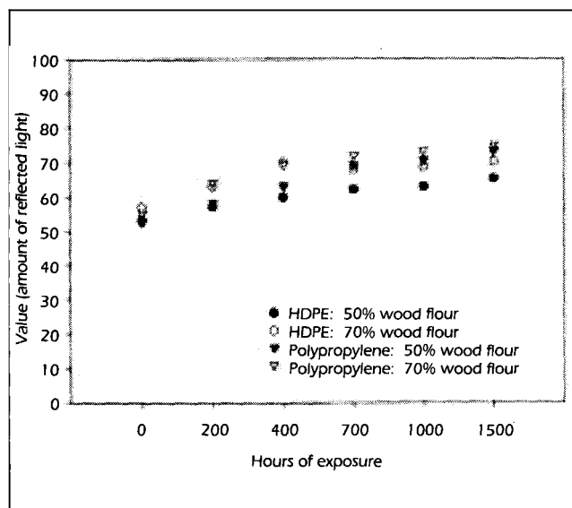
1. Effect of weatherometer exposure on color fade of unpigmented wood flour thermoplastic composites (no additives).
