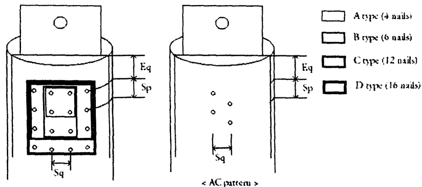
Fig. 2. Nail patterns.
