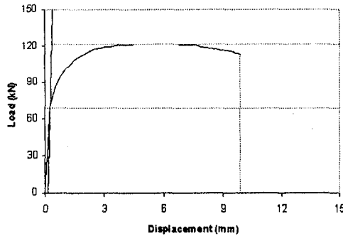
Fig. 4. Ductile failure.
