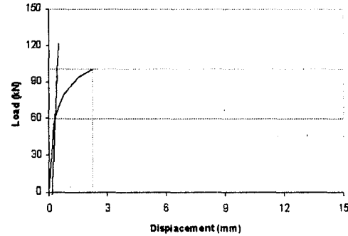
Fig. 5. Brash failure.
