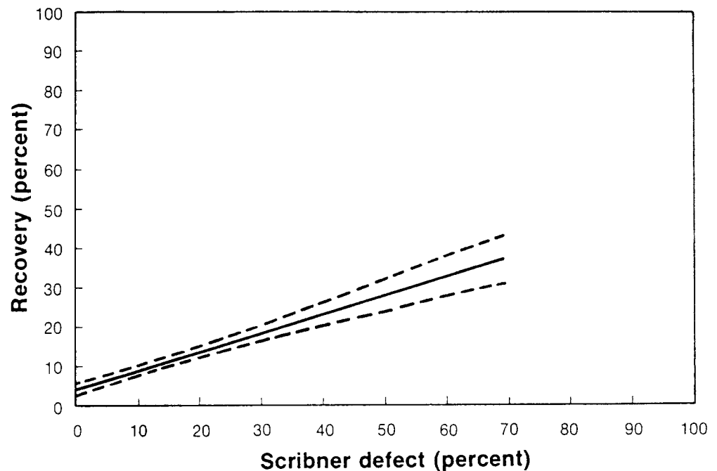
Figure 6—The relation of percent recovery of 5 Common lumber (solid line) and the 95-percent confidence intervals (dashed lines) to the percentage of Scribner scaling defect. The regression equation is shown in appendix 3.
