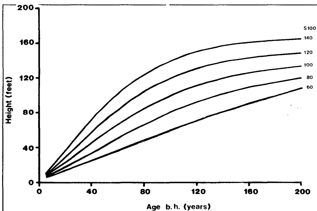
Figure 3—Height growth curves based on index age 100 years b.h., corresponding to equation (3).
