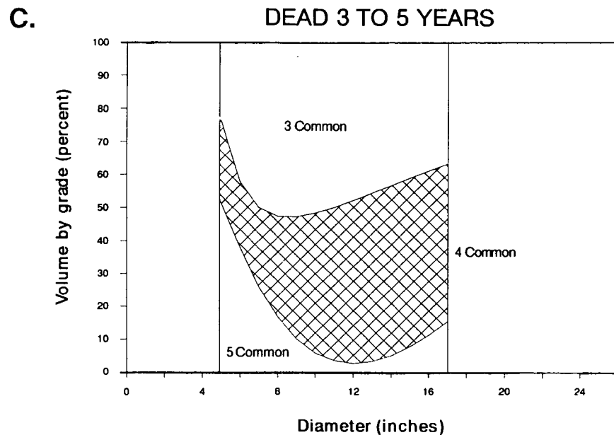
Figure 6—Cumulative percent volume by lumber grade for each of the final classes are shown. A. Moulding and Better lumber was produced only from the live sample. Because only a small portion of the mill's production was Moulding and Better, it was sold as 2 and Better Common. B. The percentage of 3 Common increased over the live sample because of blue stain. C. Because of heavy blue stain and checking, no 2 and Better Common was produced and there was a noticeable increase in 4 Common. Equations and statistics are given in table 3.
