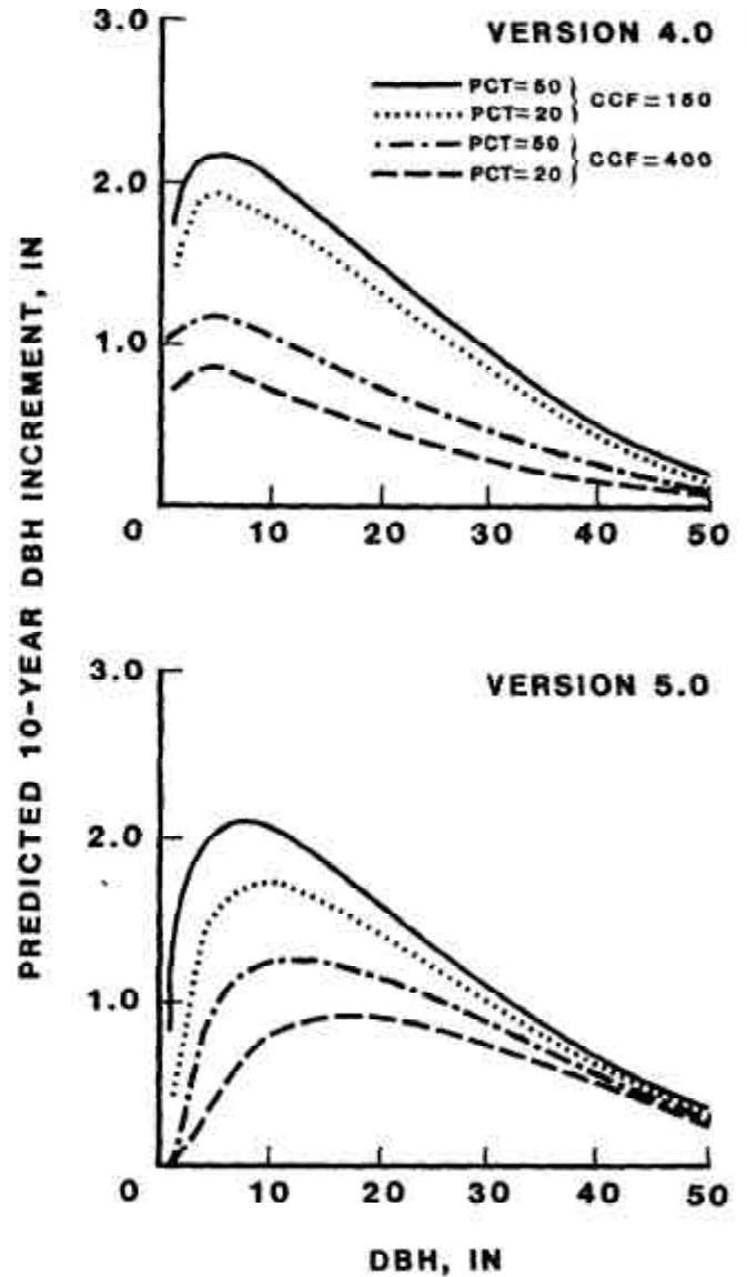
Figure 2. —The most notable differences in large-tree d.b.h. increment predictions are for subordinate trees growing in dense stands. As stand density increases, and as percentile in the basal area distribution decreases, the maximum in the increment curve shifts downward to correspond with larger d.b.h. Conditions displayed are identical to those displayed in Wykoff and others (1982; fig. 29; p. 63).
