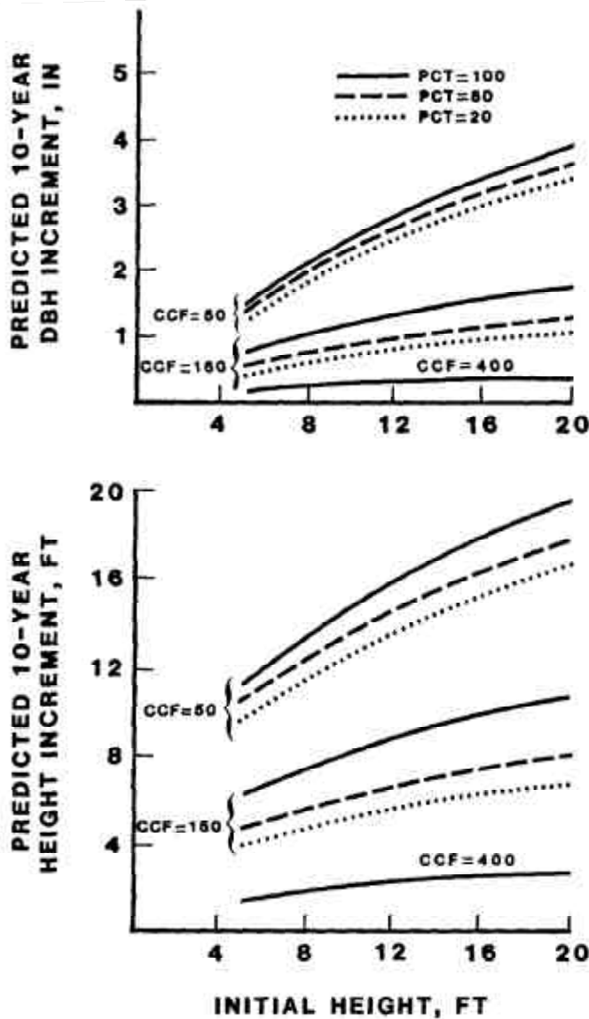
Figure 1. —Height and diameter increment predictions for small trees are sensitive to social position (as indicated by percentile in the basal area distribution, PCT) and to overall stand density (crown competition factor, CCF). Curves shown are for Douglas-fir growing on a western redcedar/Clintonia habitat type at 3,700 ft elevation in the Clearwater National Forest.
