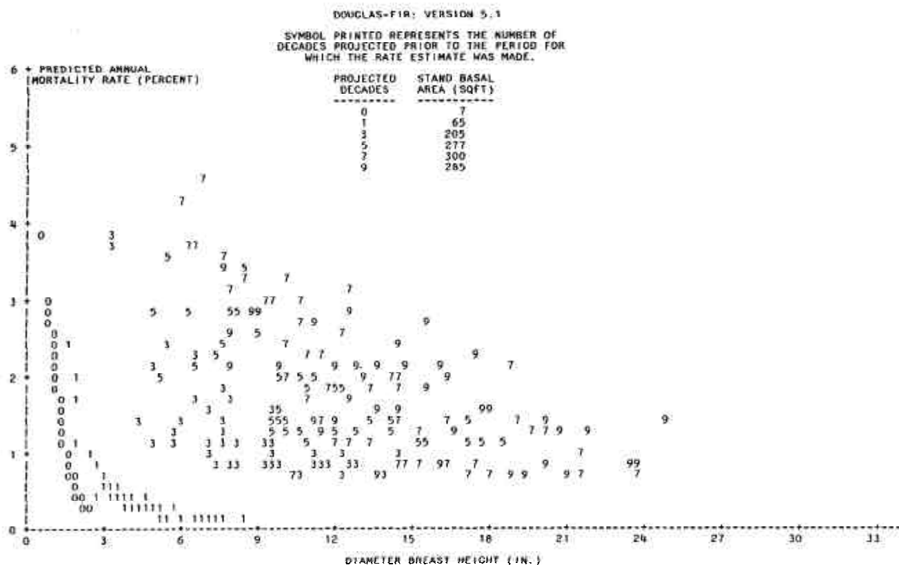
Figure 3. —Predicted annual mortality rate versus d.b.h. for Douglas-fir. The numbers printed represent decades in a long-term projection (1 is the average rate for years 11-20 in the projection; 9 is the average for years 90-100 in the projection.) Initial stand and site conditions are the same as for figure 1. Figure 3a displays rates projected by version 4.1; figure 3b displays rates projected by version 5.1.
