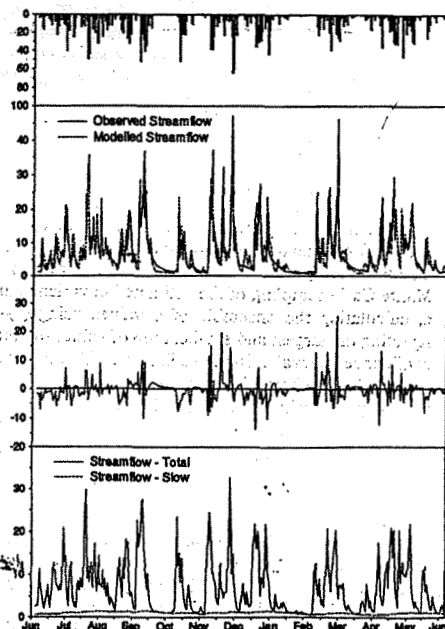
Fig. 5. Rainfall (millimeters), model fit, residuals and total/slow separation for daily streamflow (millimeters) at Kirkton in 1985-1986.
