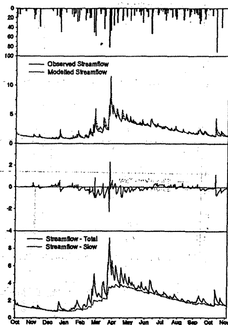
Fig. 7. Rainfall (millimeters), model fit, residuals and total/slow separation for daily streamflow (millimeters) at Coweeta watershed 34 in 1981-1982.
