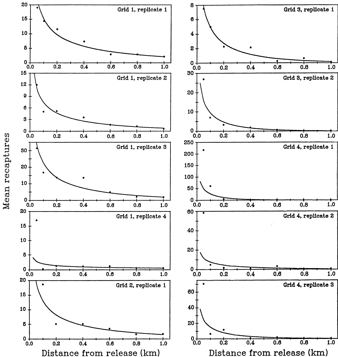
FIG. 3. Recaptures-with-distance curves for each replicate release. The data points are \bar{C}_{rj} , cumulative recaptures averaged over all traps r km from release. The solid lines are fitted curves (Eq. 6).
