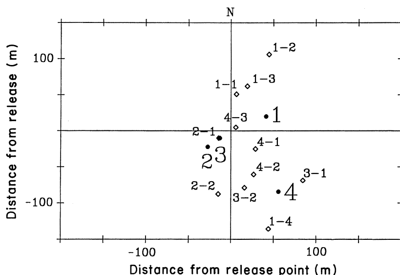
FIG. 2. Directionality effects. Average displacements of recaptures in each replicate release are indicated by \diamond . The first number at each diamond represents the number of the spatial grid, while the second number indicates the temporal replicate within each spatial grid. \bullet with large numbers indicate weighted first moments of the spatial distribution of hosts in each of four grids (see Results and discussion: Spatial heterogeneity ).
