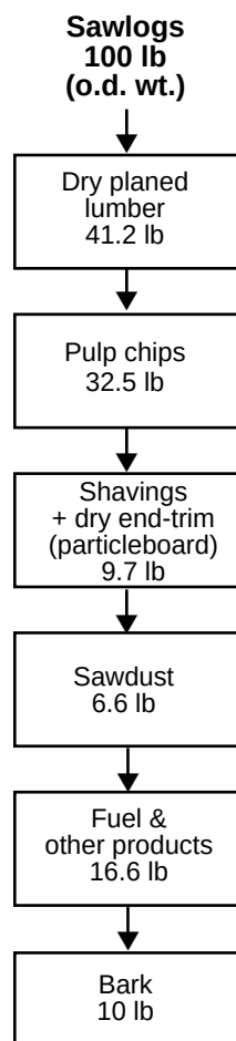
Random-length dimension lumber
