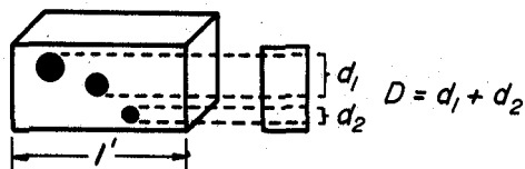
Figure 7.—Assumed cross-sectional area of knots in 7-foot interval of unit depth projected on end of the interval.
