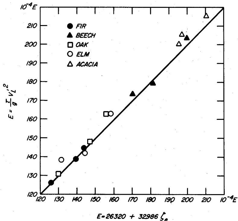
Figure B3.--Plot of coupled oscillation derived E prediction of ultrasonic modulus of elasticity (Popescu (61)).
