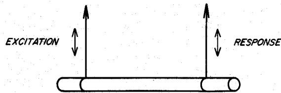
Figure 4.--Diagram showing the method of suspending a transverse vibration test specimen.
