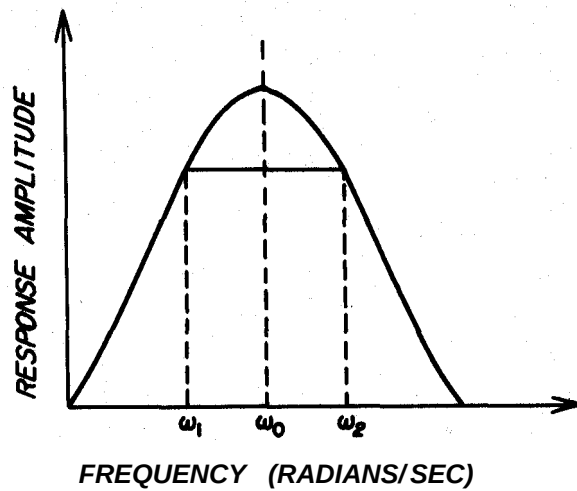
Figure 3.--Frequency response curve obtained from forced vibration.
