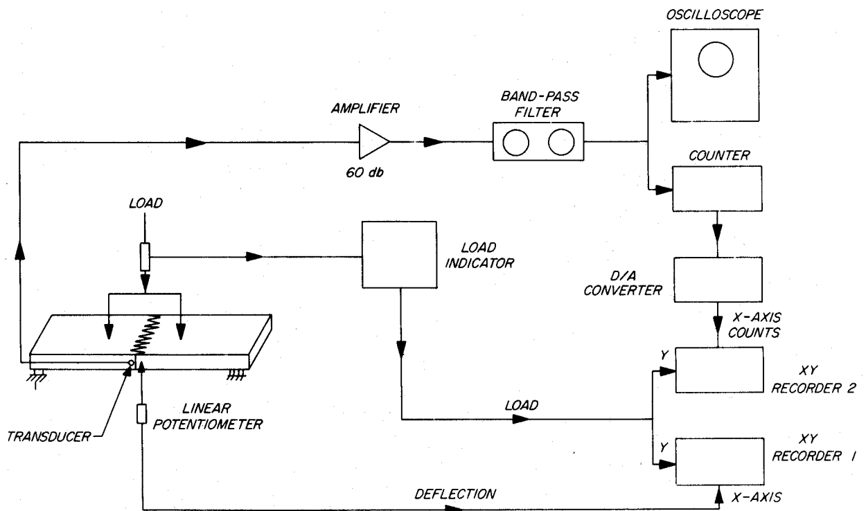
Figure B6.--Schematic representation showing the acoustic emission set up used by Porter et al. (64).
