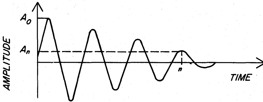
Figure 5.--Free transverse vibration decay envelope.
