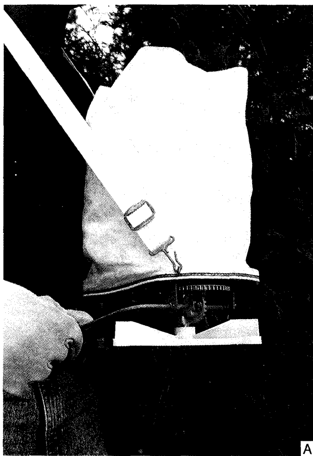
Figure 5.— (A) sack-type and (B) plastic hopper model of hand-cranked spreaders.
