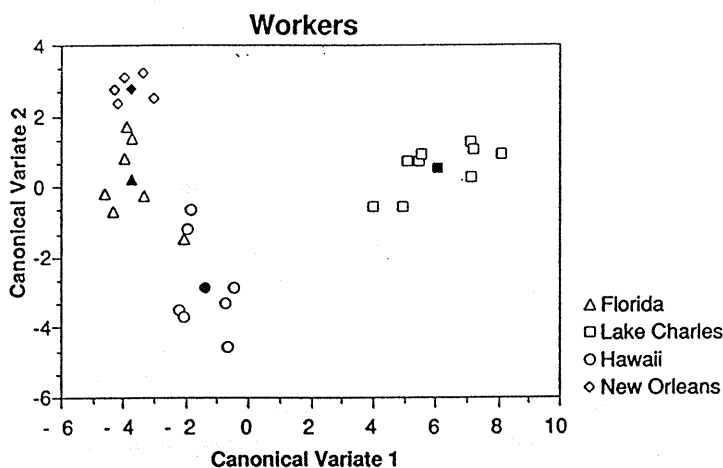
Figure 4—Plot of colonies of C. formosanus from four different locations along two axes of canonical discriminant space. Open characters represent actual data points; closed characters represent the mean value for the population.
