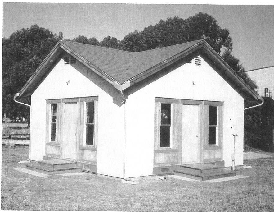
Figure 1. Villa Termiti used to test fumigation techniques and alternatives to fumigation for control of drywood termites. The Villa Termiti is symmetrical with all four sides structurally identical.
