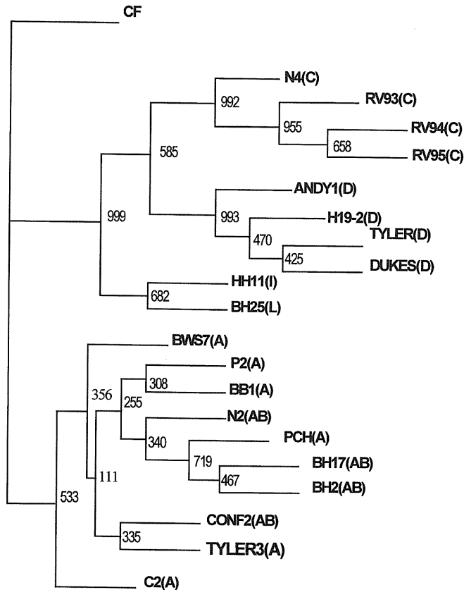
FIG. 5. Rooted maximum parsimony (MP) cladogram (Felsenstein, 1993) comparing consensus sequences, fragment of 312 segregating sites (Jenkins et al., 1999a). Numbers at the nodes were generated with SEQBOOT (Felsenstein, 1993) and represent the number of times out of 1000 the node occurred. Capital letters in parentheses represent the cuticular hydrocarbon phenotypes for the specific inspection port.
