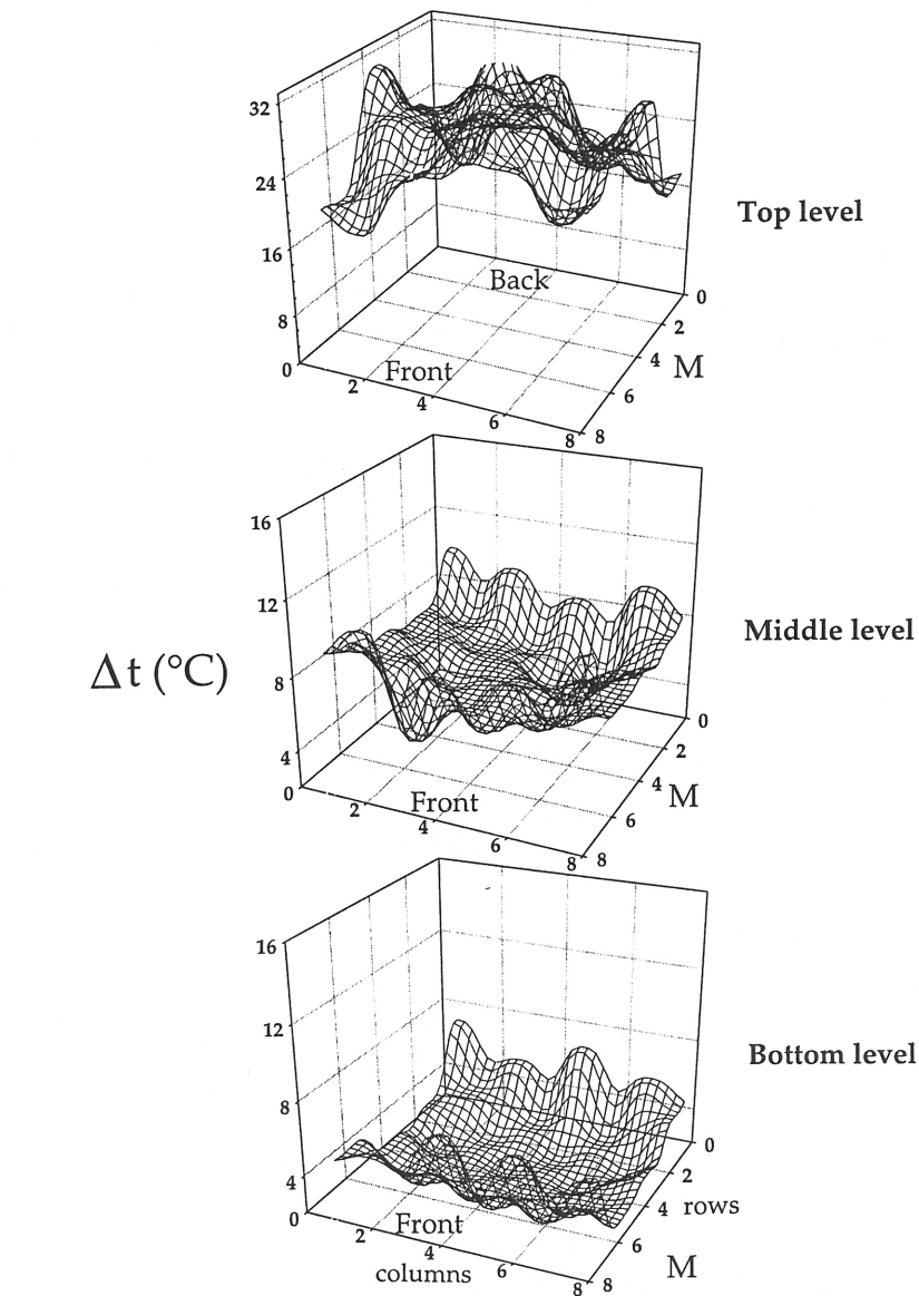
Figure 5. — 3-D plot of change in temperature ( \Delta t ) among 96 sampling locations within a 1,000-W oven. Sampling locations consisted of 25-mL vials filled with water and heated at full power for 2 minutes. M denotes the location of the megatron, the source of microwave emissions.
