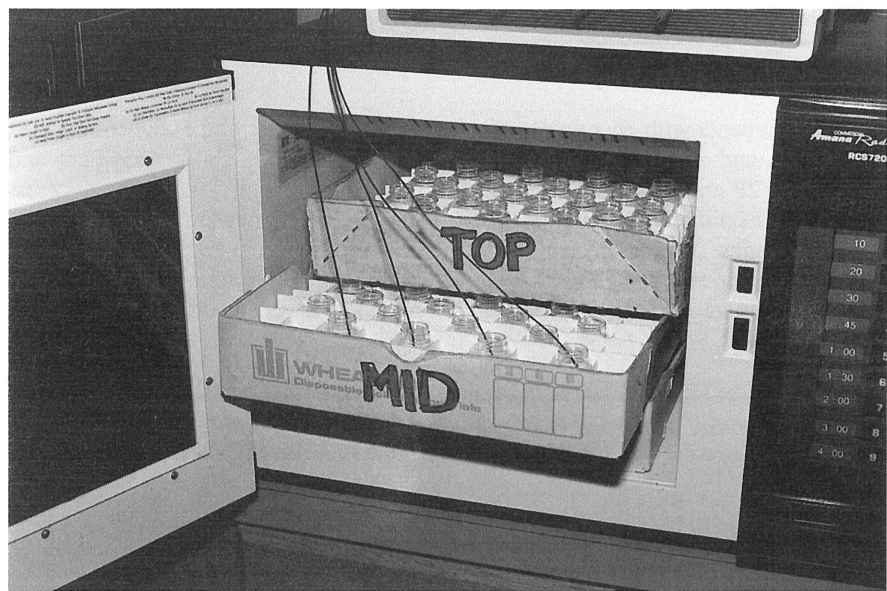
Figure 2. — Two vertically stacked cardboard trays containing 64 25-mL water-filled vials. Ovens producing 500-W, 1,000-W, and 2,000-W were run at full power for 4 minutes, 2 minutes, and 45 seconds, respectively. Initial and final temperature was recorded for each vial to calculate oven wattage.
