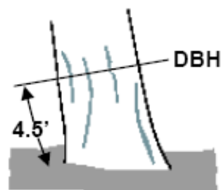
Figure 8.15: Leaning tree.
