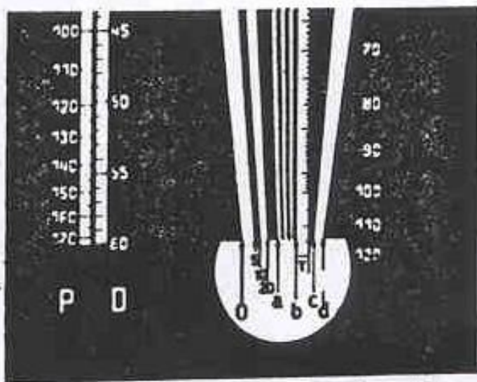
Fig. 62 Lower part of American scale, enlarged to show identification of graduations.
