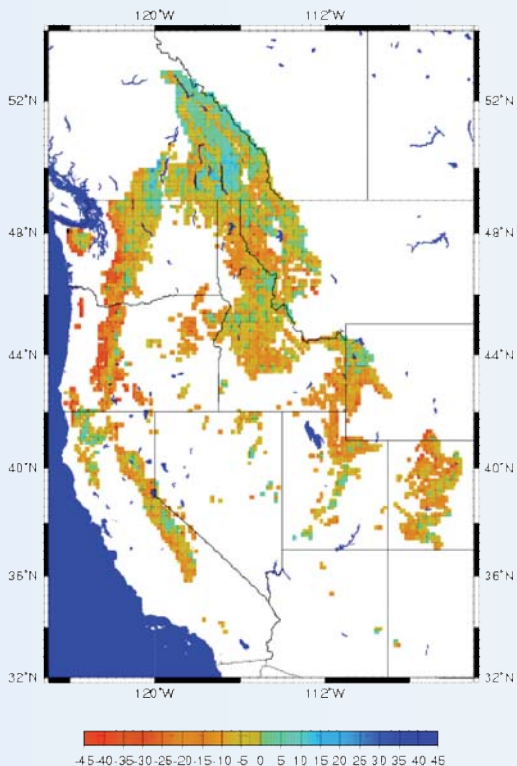
Cumulative trend in simulated timing of peak snowpack (number of days changed from 1951 to 2000).
