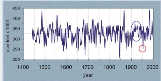
Reconstructed Colorado Headwaters Streamflow, 1437-2002 smoothed with a 5-weight filter
