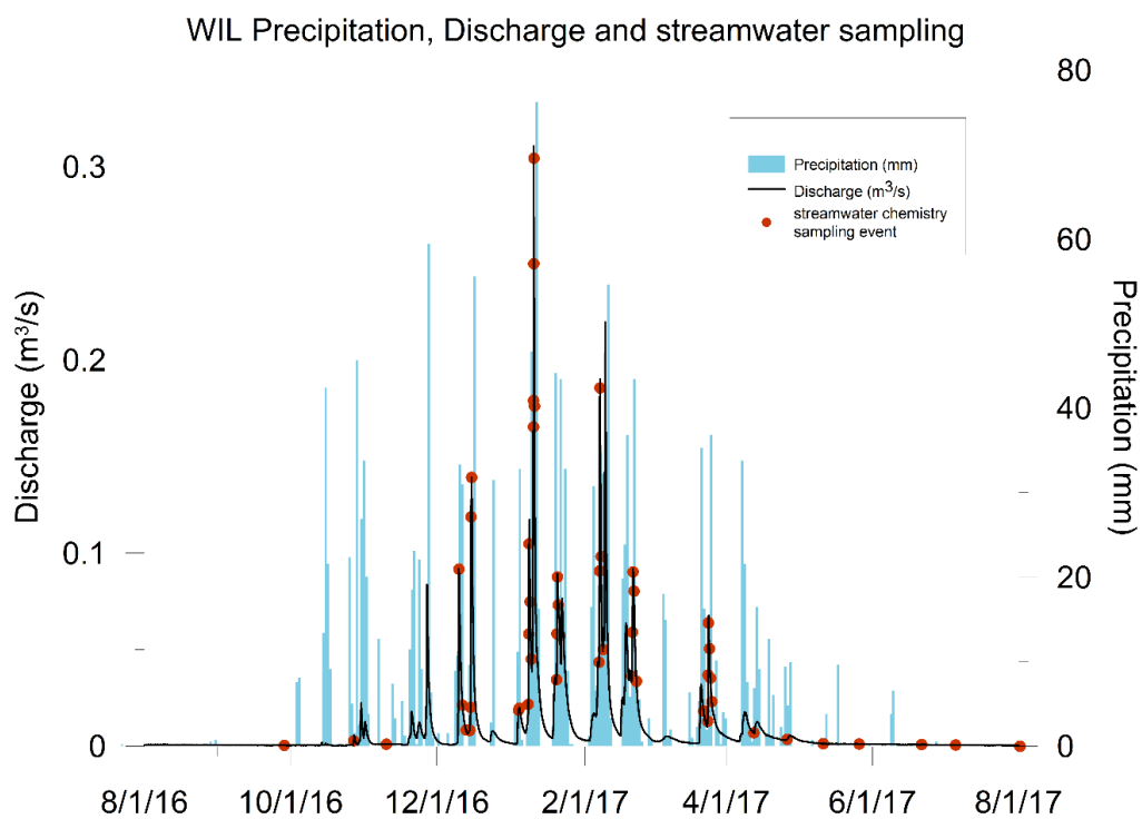
Figure 5. HY2017 WIL precipitation, discharge and sampling events.
