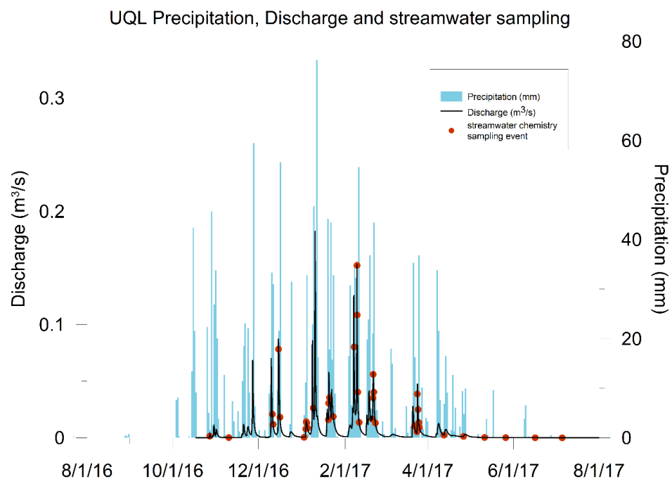
Figure 4. HY2017 UQL precipitation, discharge and sampling events.
