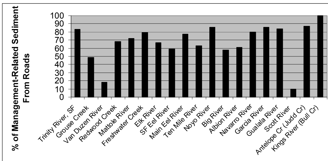
Figure 2. California sediment budgets from the northern Coast Ranges (16), Klamath Mountains (1), Cascade Range (1) and Sierra Nevada (1), showing the percent of management-related sediment estimated to derive from forest roads. The Redwood Creek sediment budget includes roads and skid trails; 68 percent of sediment for the Antelope Creek (Judd Cr.) sediment budget is estimated to result from long-term post-fire surface erosion; 14 of the 19 sediment budgets displayed were produced as part of TMDL documents for watersheds listed as impaired by the U.S. EPA.
