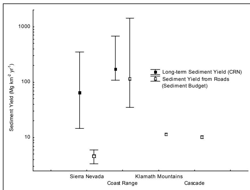
Figure 3. Comparison of millennial averaged sediment production rates derived from cosmogenic radio nuclide dating (CRN) to short-term sediment yields derived from sediment budgets produced for California watersheds. The boxes represent the median value and the error bars represent the range of values. CRN data is not available for the Klamath Mountains and the Cascade Range.
