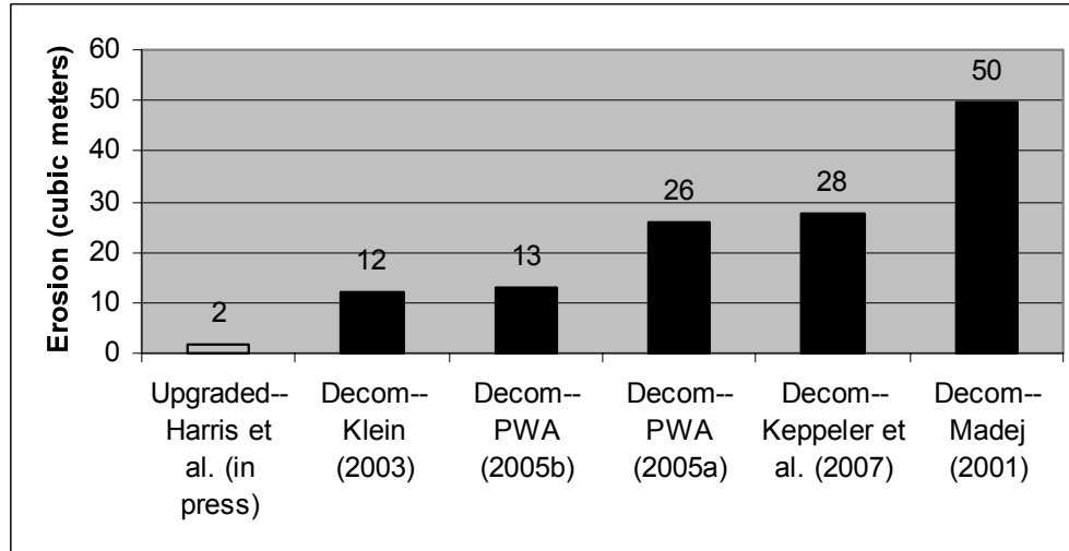
Figure 4. Comparison of post-treatment erosion volumes from decommissioned versus upgraded watercourse crossings.
