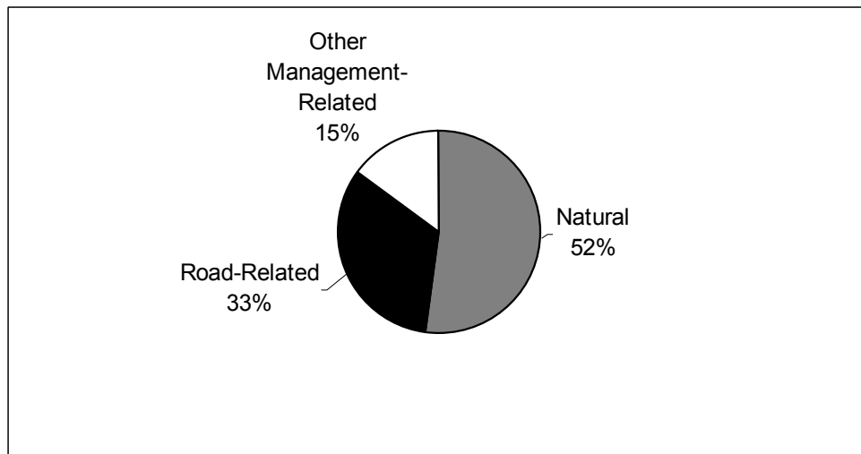
Figure 1. Distribution of natural and management-related sediment from 19 sediment budgets located in California.
