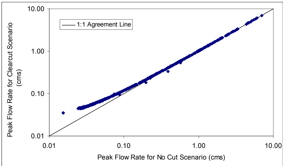
Figure 6-7. Modeled changes in peak flow rate for harvested vs. un-harvested forest management scenarios in North Fork Caspar Creek, CA.
