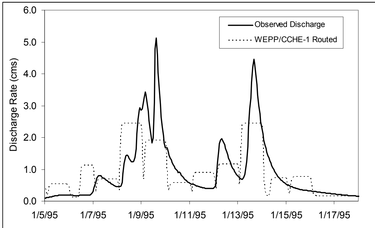
Figure 3-7. Observed discharge at South Fork Caspar Creek (January 3-18, 1995) vs. Predicted discharge (simulated with WEPP/CCHE-1).
