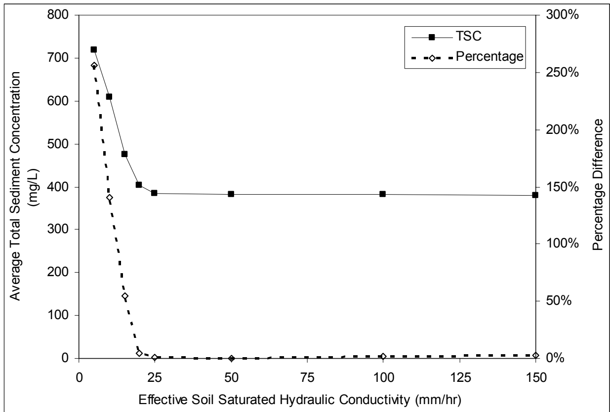
Figure 5-19. Differences in total sediment concentration for changes in soil saturated hydraulic conductivity at South Fork Caspar Creek, CA.
