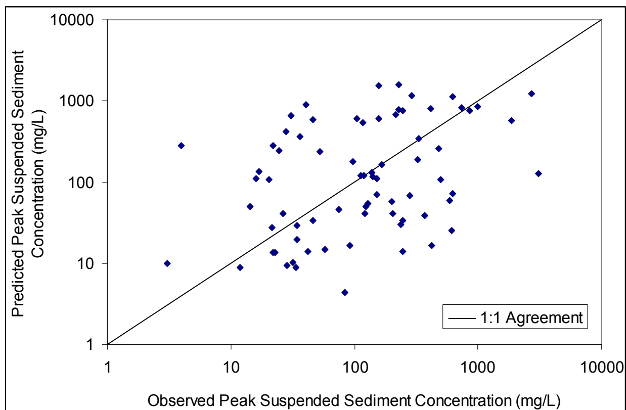
Figure 4-2. Predicted vs. observed peak daily suspended sediment concentration for South Fork Caspar Creek simulation (1995-1997).
