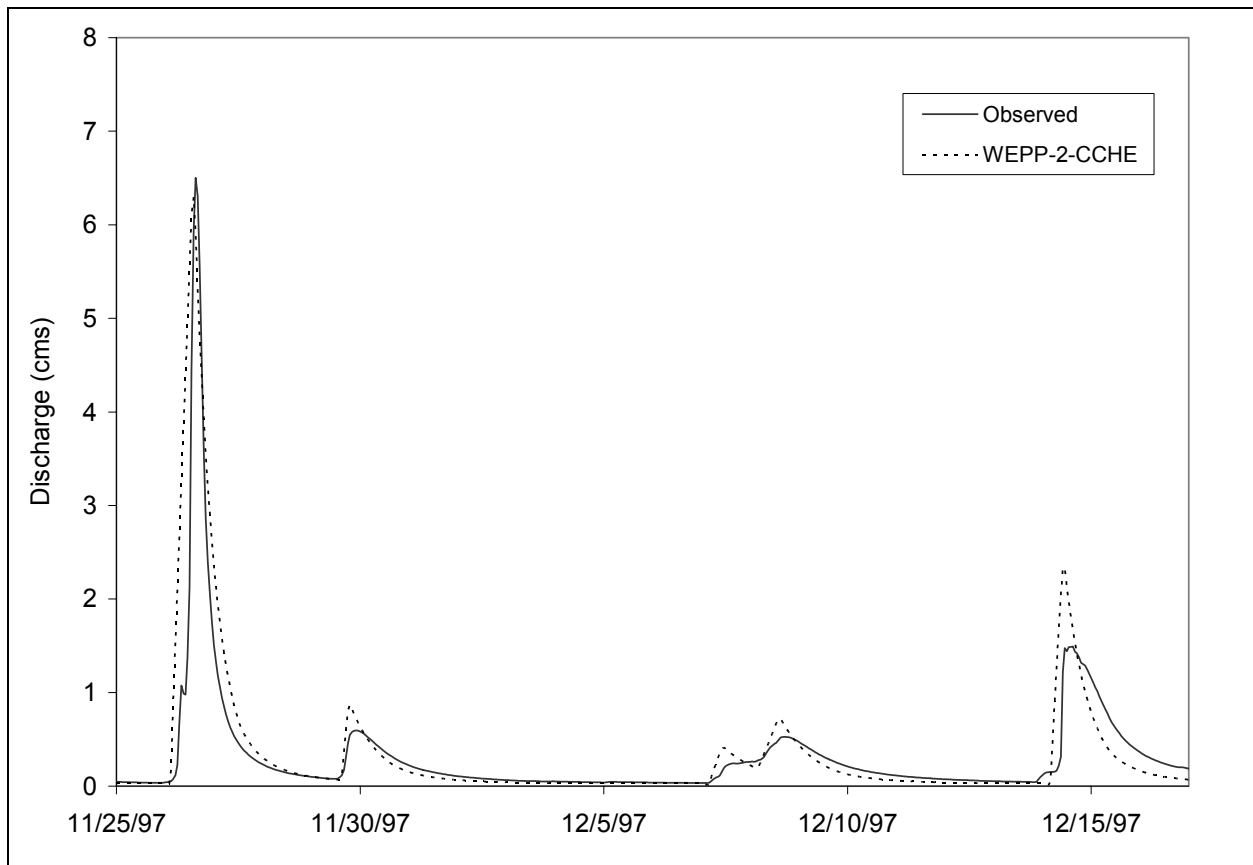
Figure 5-2. Observed and predicted discharge for South Fork Caspar Creek, CA, for the period of November 26, 1997 thru December 17, 1997.
