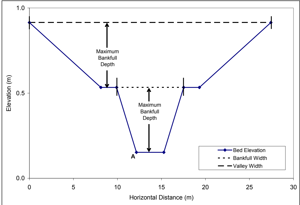
Figure 3-4. Schematic diagram of generated channel geometry.
