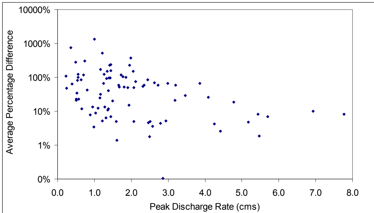
Figure 5-22. Percent difference in peak discharge rate by peak discharge rate for South Fork Caspar Creek, CA.
