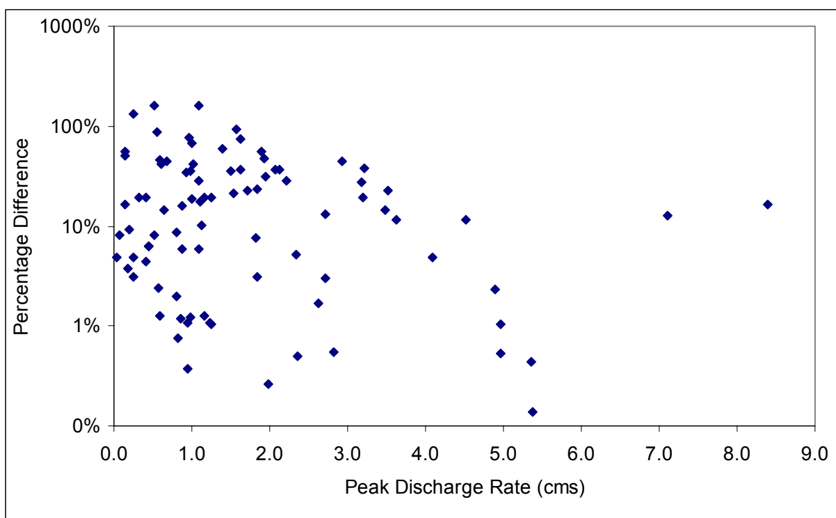
Figure 5-18. Percentage change in peak discharge rate for given peak discharge rates at South Fork Caspar Creek, CA.
