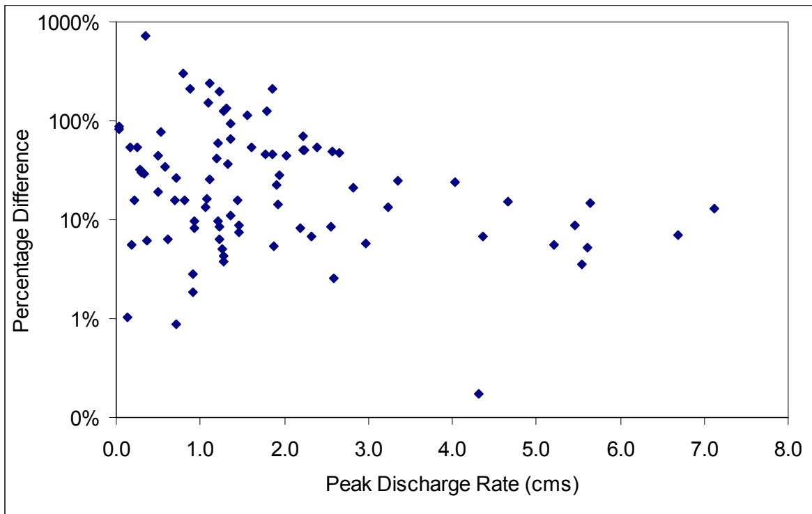
Figure 5-24. Percentage difference in predicted peak discharge rate for given peak discharge rates at South Fork Caspar Creek, CA.
