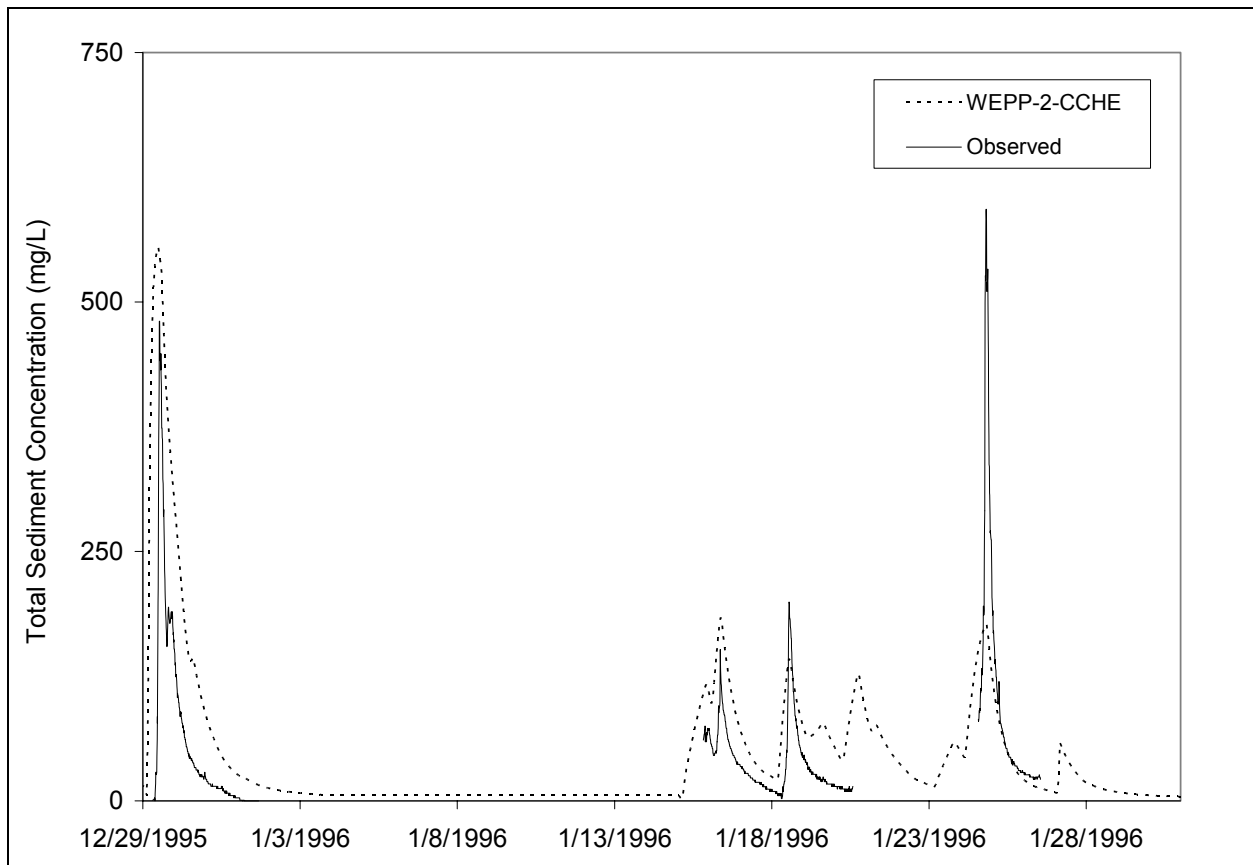
Figure 5-3. Observed and predicted total sediment concentration for South Fork Caspar Creek, CA, for the period of December 29, 1995 thru January 29, 1996.
