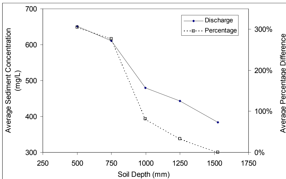
Figure 5-21. Percentage difference in total sediment concentration for changes in soil depth in South Fork Caspar Creek, CA.
