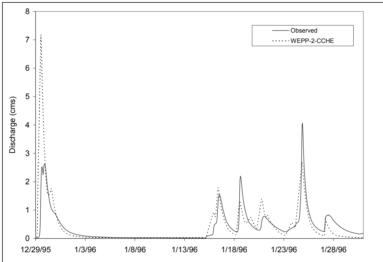
Figure 5-1. Observed and predicted discharge for South Fork Caspar Creek, CA, for the period of December 29, 1995 thru January 31, 1996.
