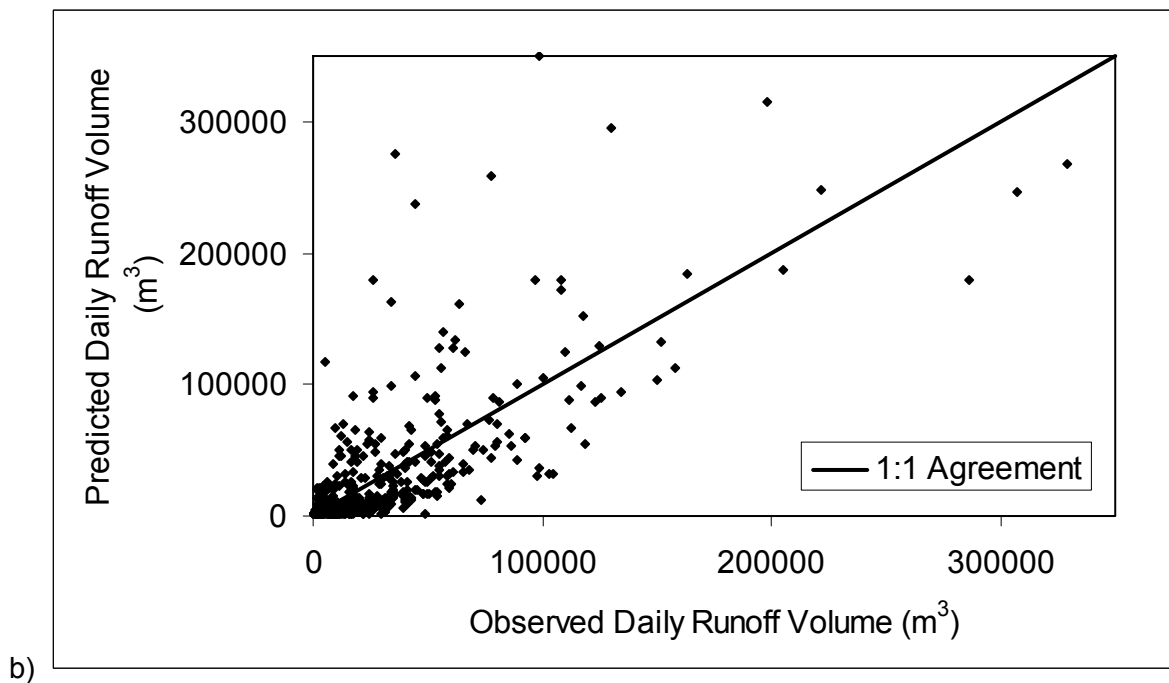
Figure 6-5. Observed vs. predicted daily runoff volumes for North Fork Caspar Creek (1986-1995), a) logarithmic axes, b) arithmetic axes.
