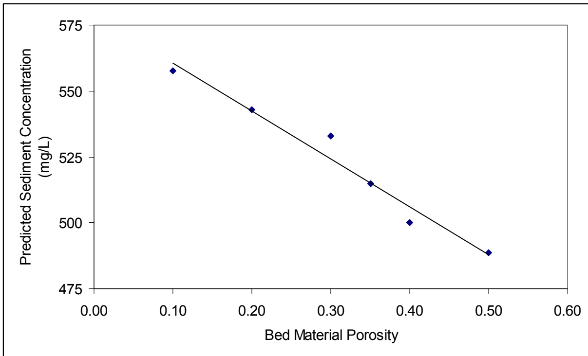
Figure 5-14. Predicted total sediment concentration for varying bed material porosity levels.
