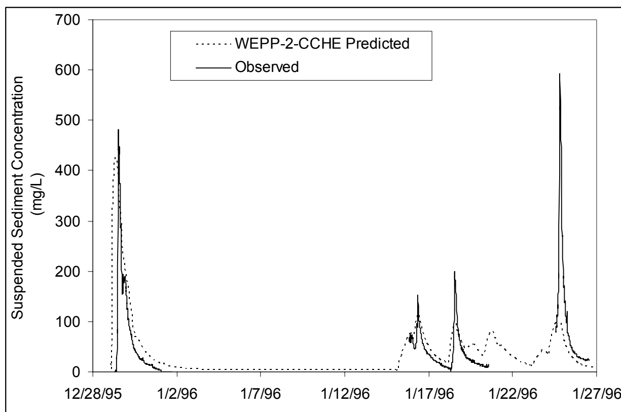
Figure 4-1. Observed and predicted suspended sediment concentration at South Fork Caspar Creek, CA, December 1995 thru January 1996.
