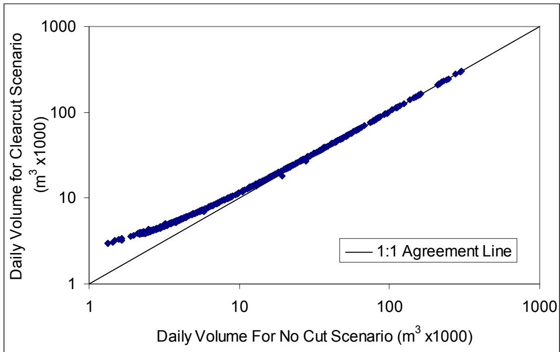
Figure 6-9. Modeled changes in daily flow volume for harvested vs. un-harvested forest management scenarios in North Fork Caspar Creek, CA.
