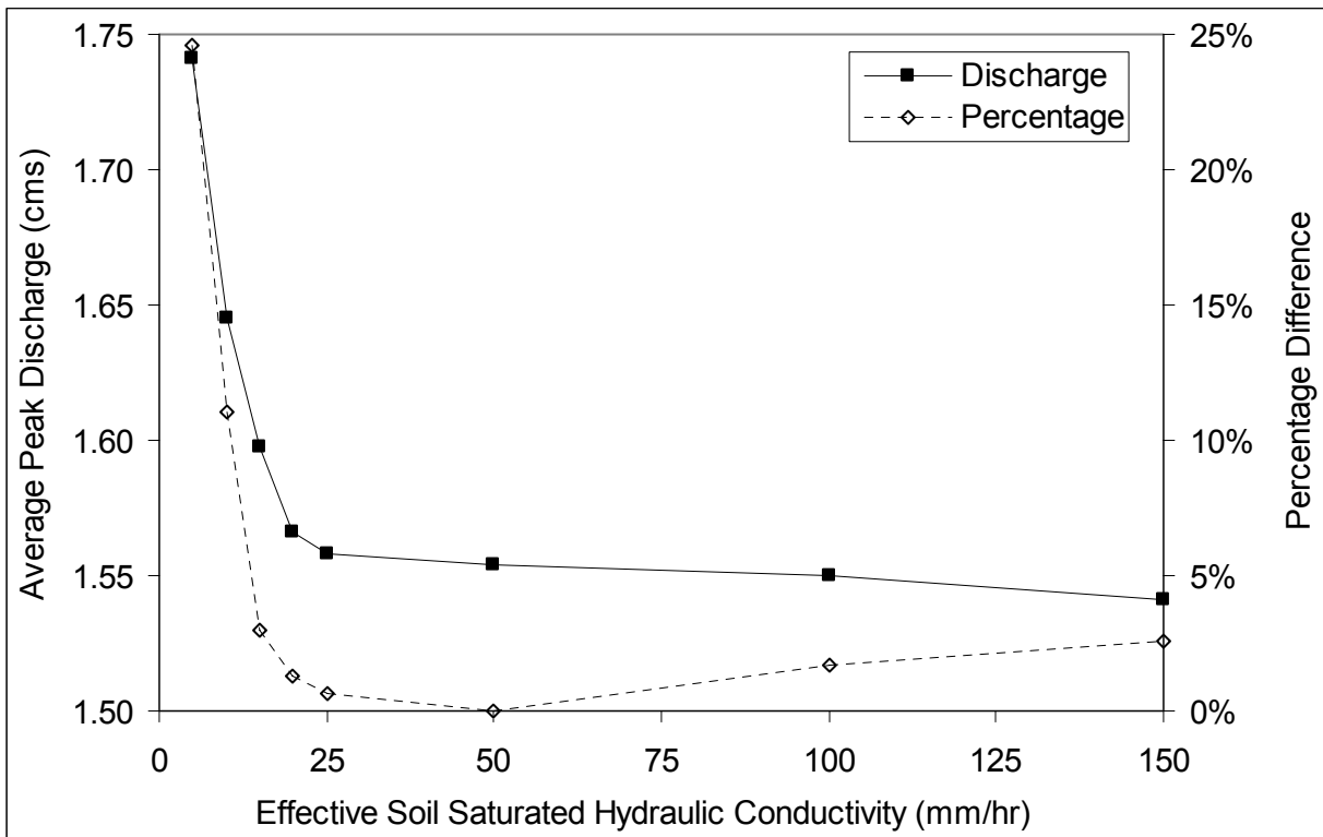
Figure 5-17. Differences in discharge rates for changes in soil saturated hydraulic conductivity at South Fork Caspar Creek, CA.
