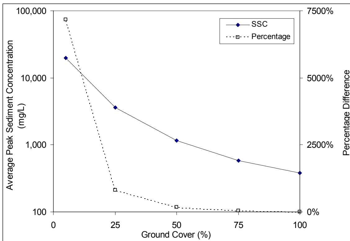
Figure 5-25. Changes in average peak sediment concentration (with percentage difference from 100% cover) for changes in percentage ground cover, simulated at South Fork Caspar Creek, CA.
