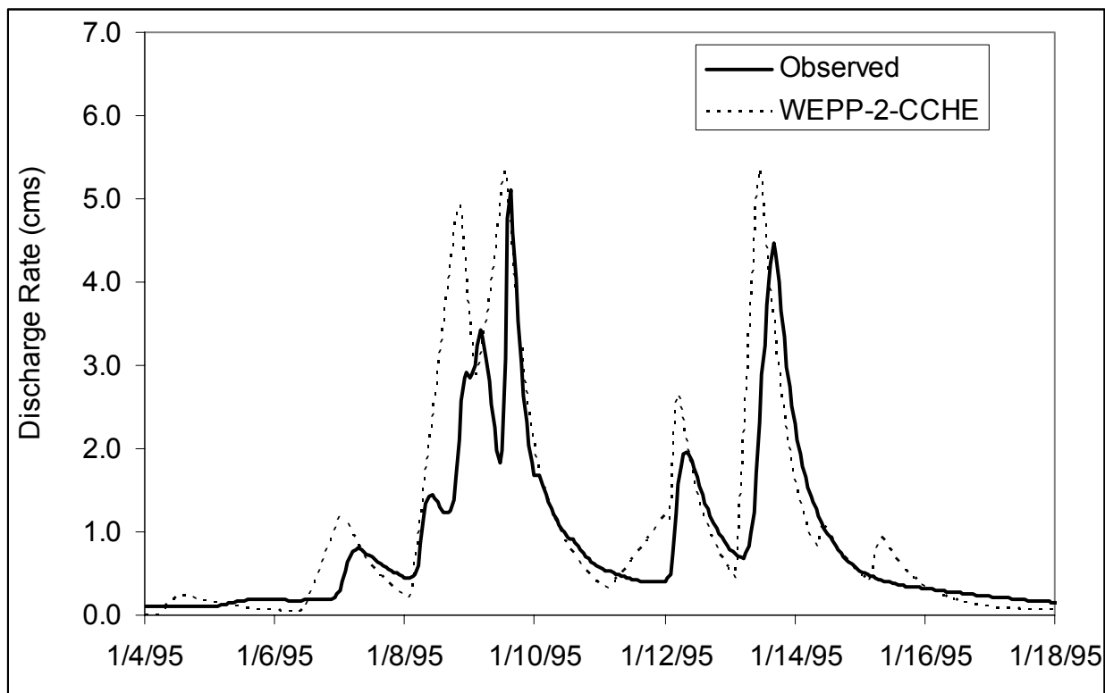
Figure 3-8. Observed discharge at South Fork Caspar Creek (January 3-18, 1995) vs. Predicted discharge (simulated with WEPP-2-CCHE).
