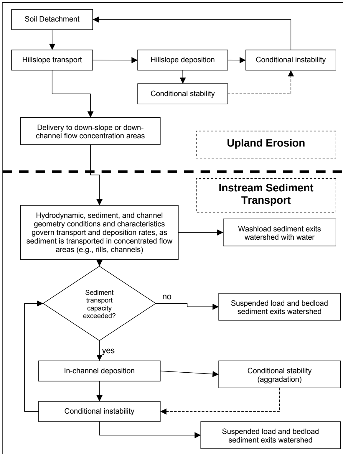
Figure 2-1. Schematic of watershed-scale erosion processes.
