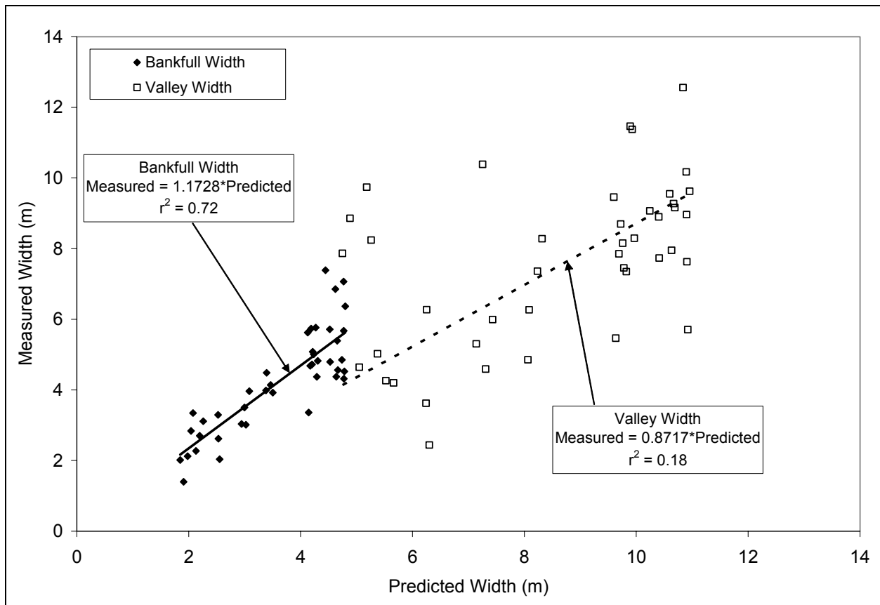
Figure 3-2. Measured vs. predicted bankfull and valley width for 42 stream channel cross-sections in North Fork Caspar Creek, CA. Predicted values were computed with Equations 1 and 2, respectively.
