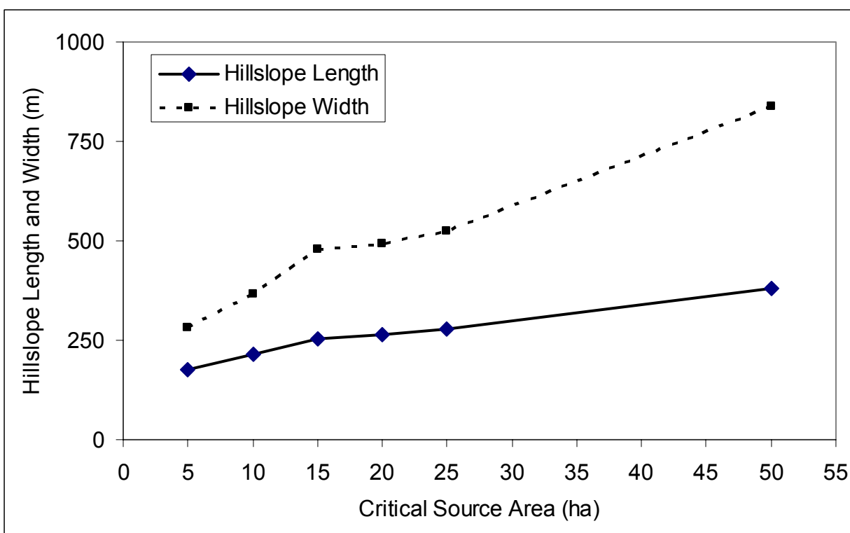
Figure 6-3. Hillslope length and width for varying critical source areas.
