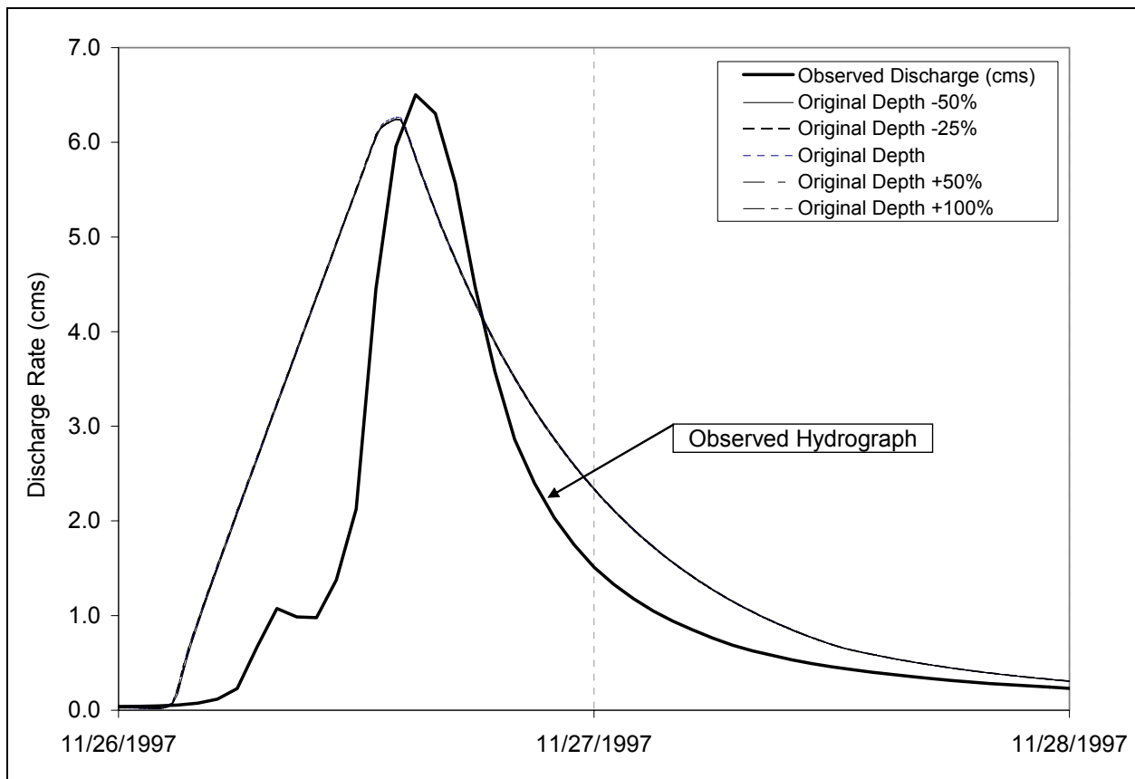
Figure 5-6. Example hydrographs for an event with channel cross-section depth changed from originally modeled value.
