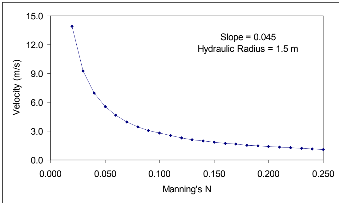
Figure 5-12. Variations in streamflow velocity for uniform flow in a trapezoidal channel with varying Manning's roughness coefficient.
