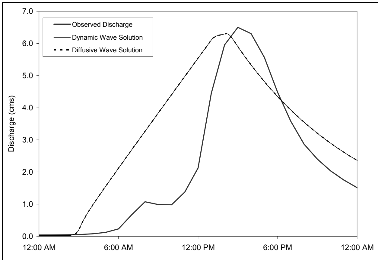
Figure 5-15. Example differences in hydrographs for dynamic and diffusive wave solutions for a selected runoff event in South Fork Caspar Creek, CA.
