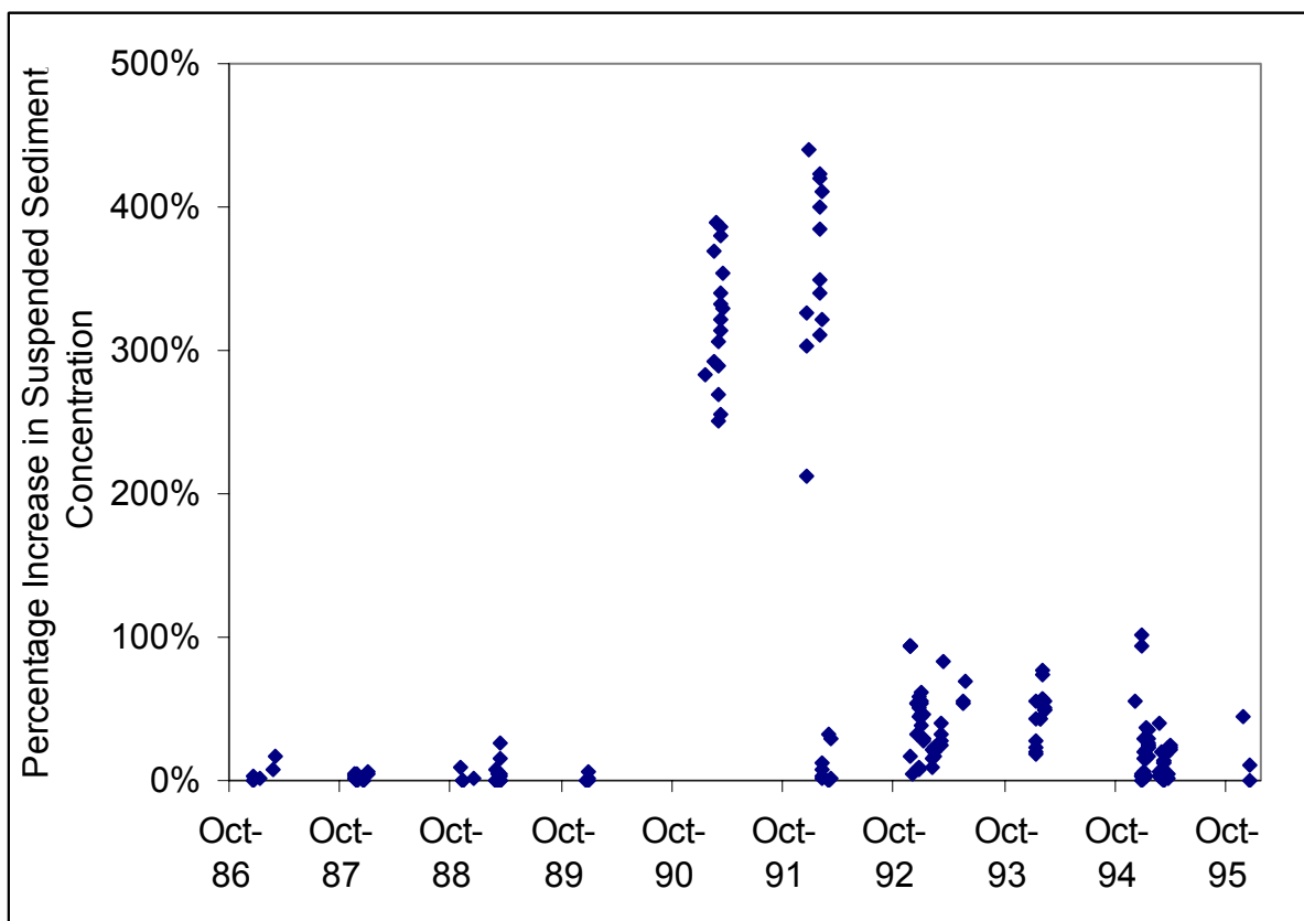
Figure 6-12. Percentage change in suspended sediment concentration between harvested and un-harvested scenarios, for North Fork Caspar Creek, CA (1986-1995).
