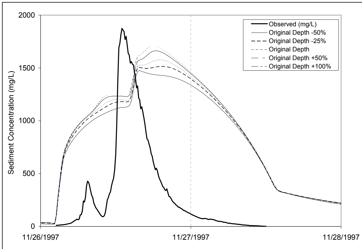
Figure 5-8. Example sediment graph for an event with channel cross-section depth changed from originally modeled value.
