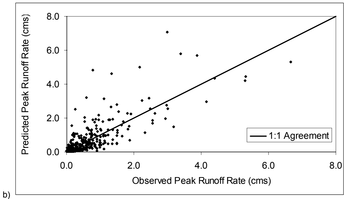
Figure 6-4. Observed vs. predicted peak runoff rates for North Fork Caspar Creek (1986-1995), a) logarithmic axes, b) arithmetic axes.
