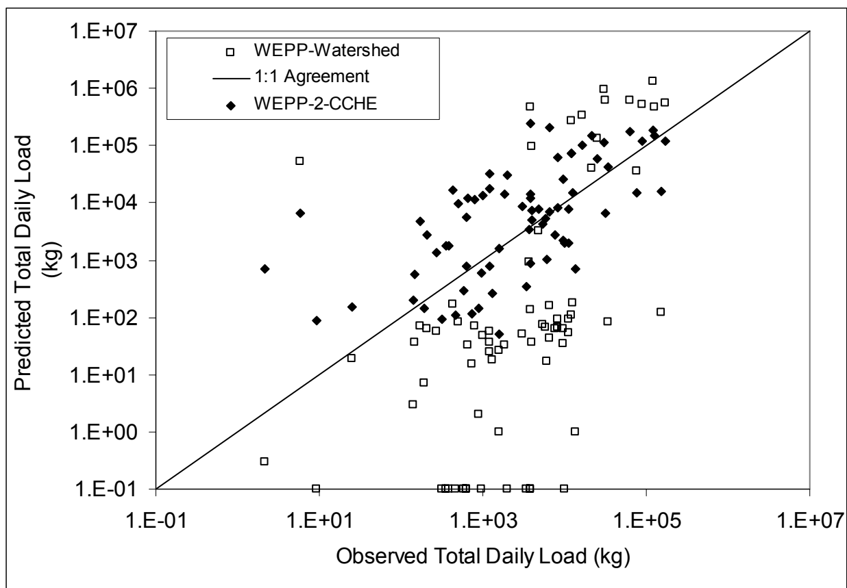
Figure 4-3. Predicted total daily sediment load (with WEPP-2-CCHE) vs. observed total daily sediment load for South Fork Caspar Creek simulation (1995-1997).
