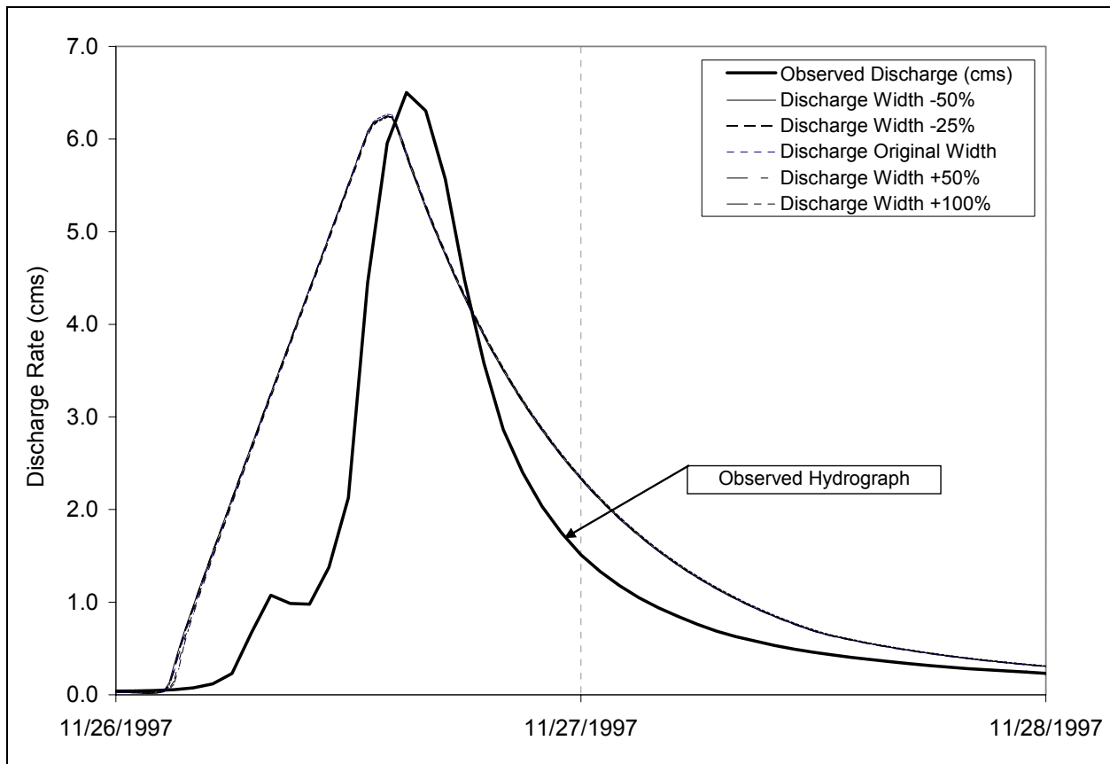
Figure 5-7. Example hydrographs for an event with channel cross-section width changed from originally modeled value.
