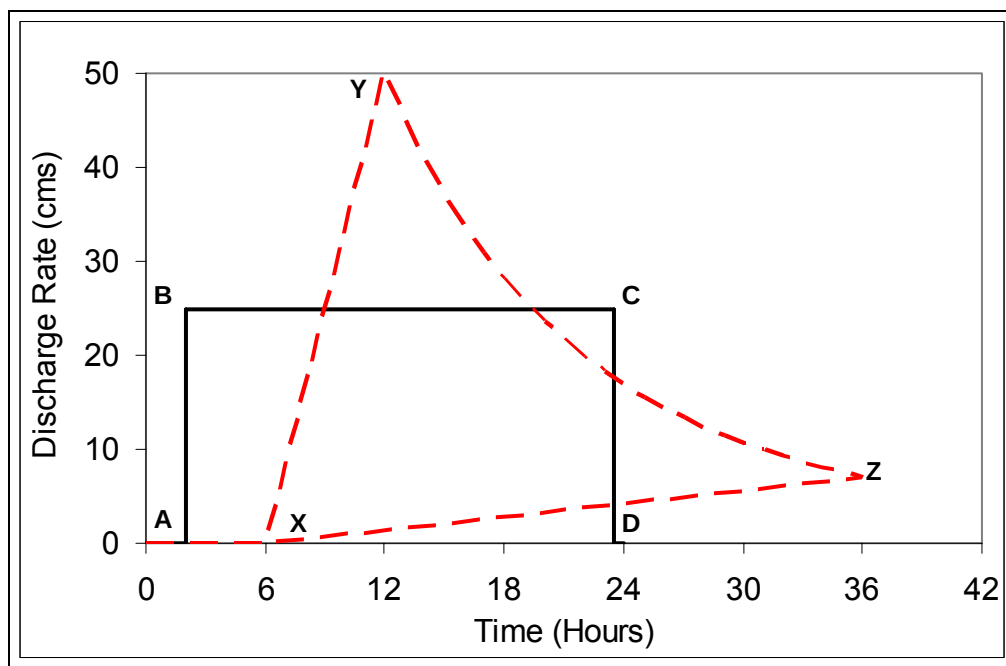
Figure 3-6. Adjusted hydrograph (dashed area X-Y-Z) with an equal volume to the rectangular hydrograph (solid area A-B-C-D).
