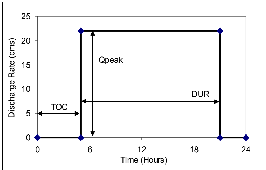
Figure 3-5. Example hydrograph created using data from WEPP Hillslope output pass file.
