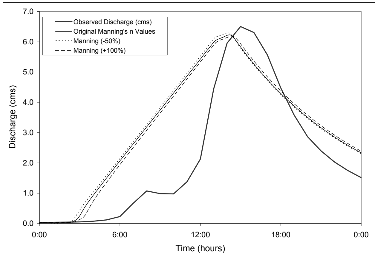
Figure 5-10. Example differences in hydrographs for increases and decreases of Manning's roughness coefficient of 100 and 50 (respectively) from originally used values for a selected runoff event in South Fork Caspar Creek, CA.
