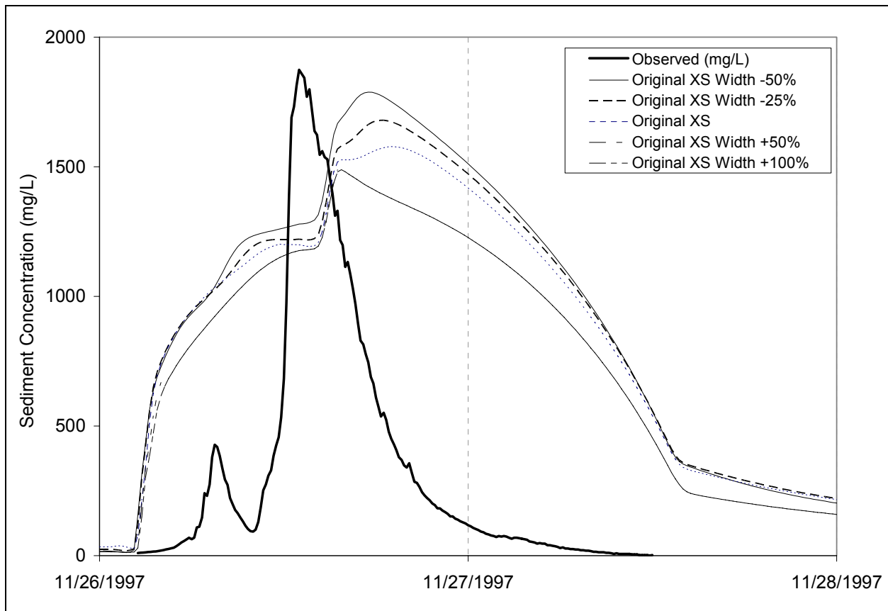
Figure 5-9. Example sediment graph for an event with channel cross-section width changed from originally modeled value.
