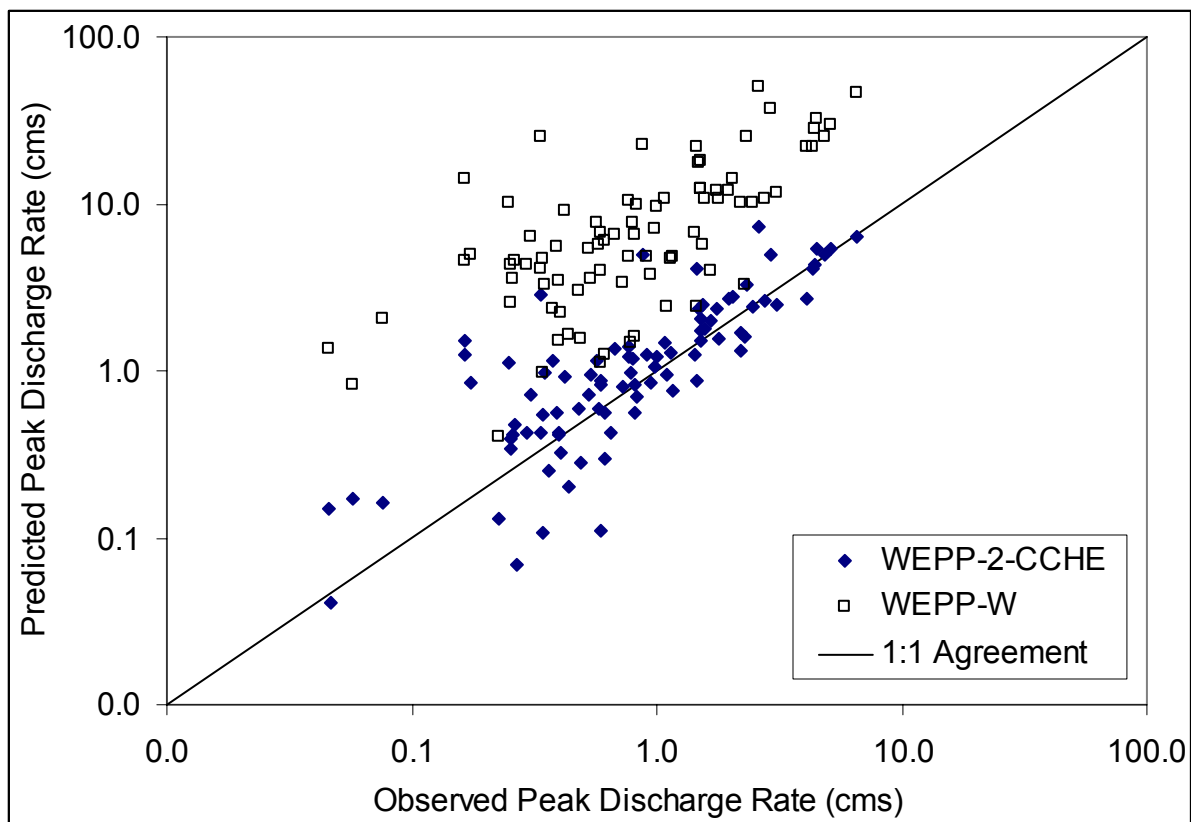
Figure 3-10. Observed vs. predicted daily peak runoff rate for 89 events at South Fork Caspar Creek Experimental Watershed, CA (1995-1997).
