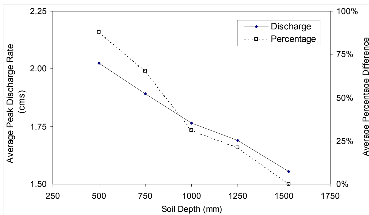
Figure 5-20. Percent difference in peak discharge rate for changes in soil depth in South Fork Caspar Creek, CA.
