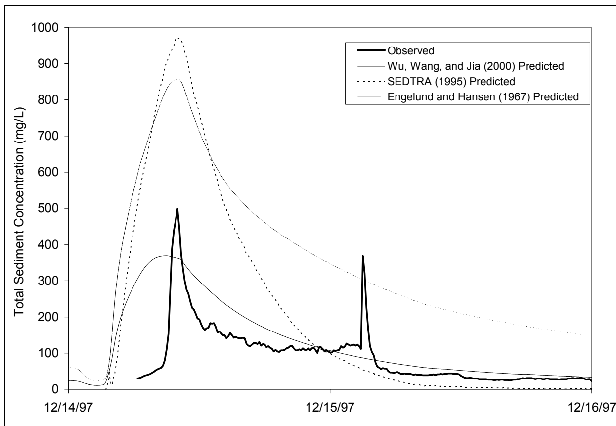
Figure 5-16. Example differences in sediment graphs for three sediment transport capacity equation options available in CCHE1D, for a selected runoff event in South Fork Caspar Creek, CA.
