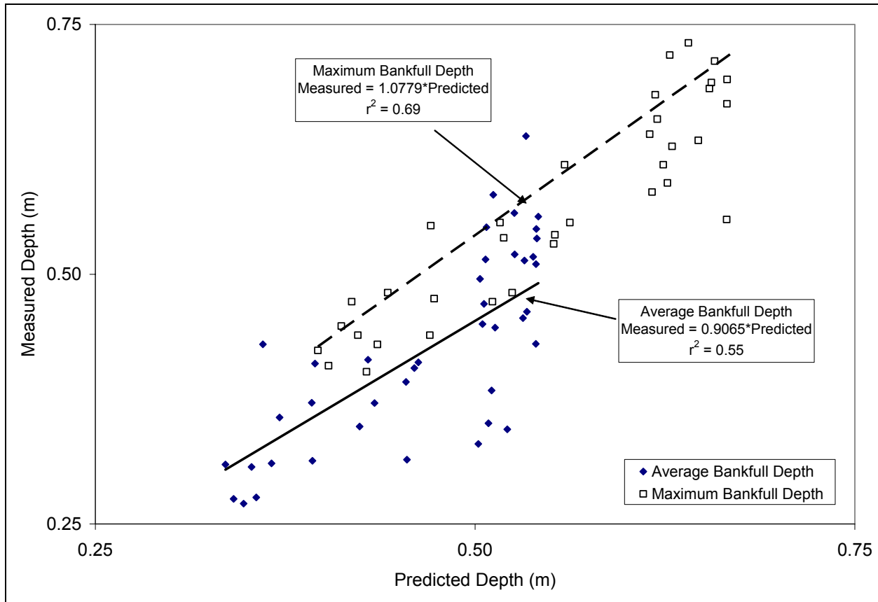
Figure 3-3. Measured vs. predicted average and maximum bankfull depth for 42 stream channel cross-sections in North Fork Caspar Creek, CA. Predicted values were computed with Equations 3 and 4.
