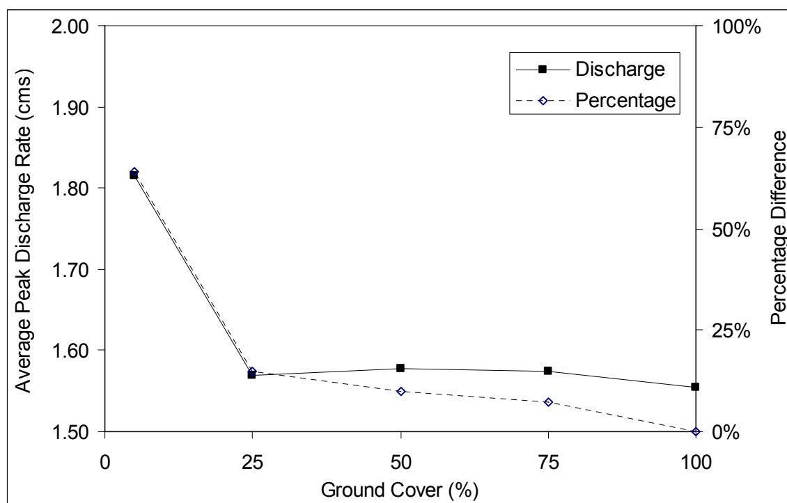
Figure 5-23. Percentage difference in average peak discharge rate (with percentage difference from 100% cover) for changes in percentage ground cover from 100% cover, simulated at South Fork Caspar Creek, CA.
