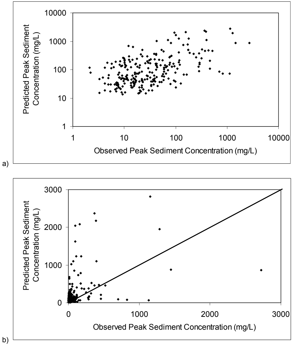
Figure 6-6. Observed vs. predicted peak sediment concentration for North Fork Caspar Creek (1986-1995), a) logarithmic axes, b) arithmetic axes.
