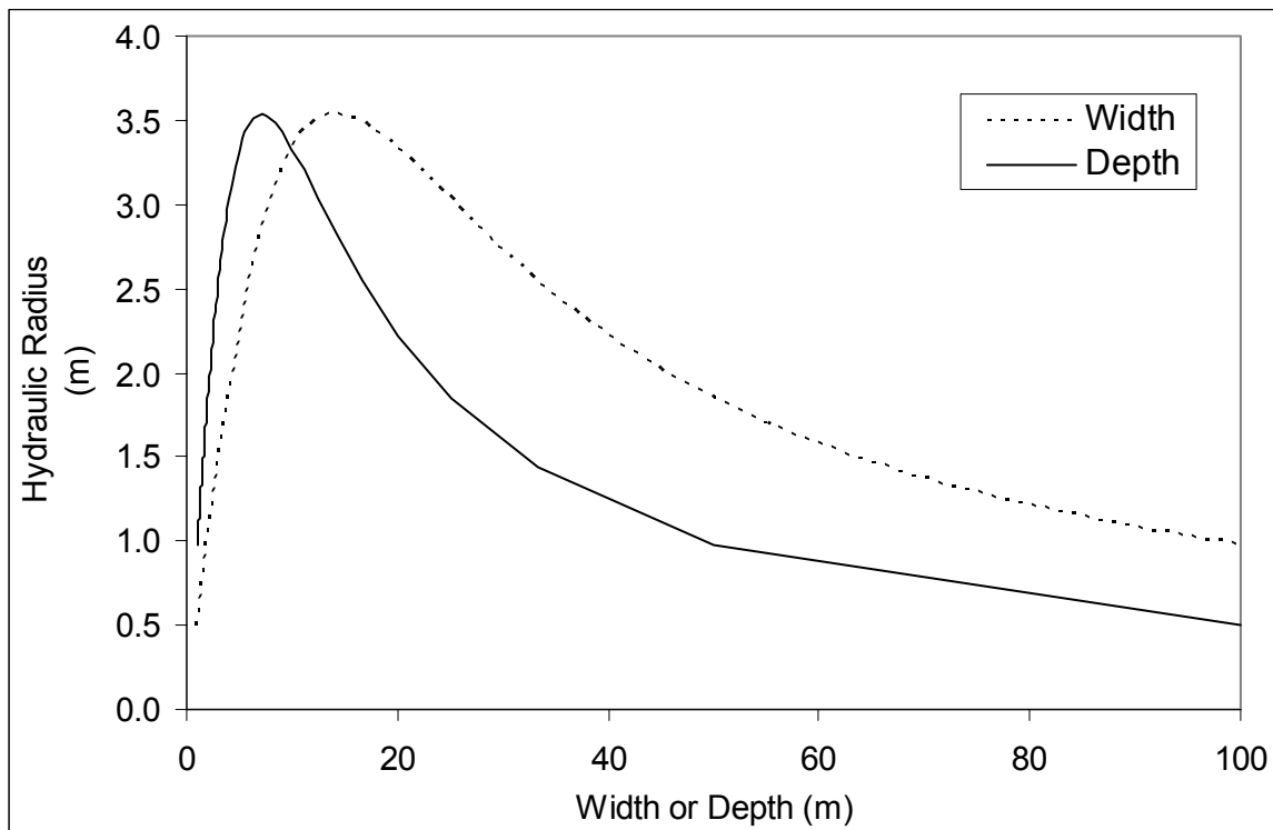
Figure 5-5. Changes in hydraulic radius of a hypothetical, rectangular channel (cross-sectional area = 100 \text{ m}^2 ) when channel width and depth are changed but area is held constant.
