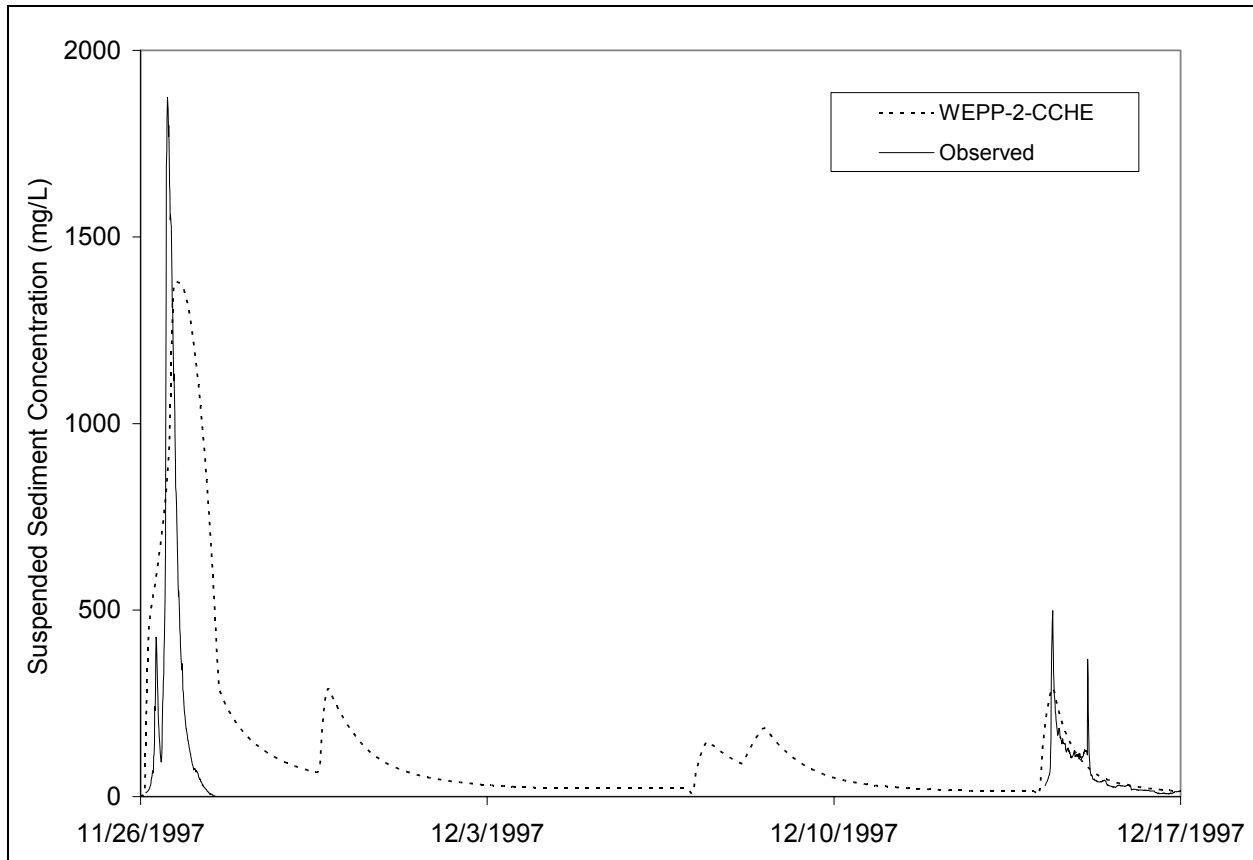
Figure 5-4 Observed and predicted total sediment concentration for South Fork Caspar Creek, CA, for the period of November 26, 1997 thru December 17, 1997.
