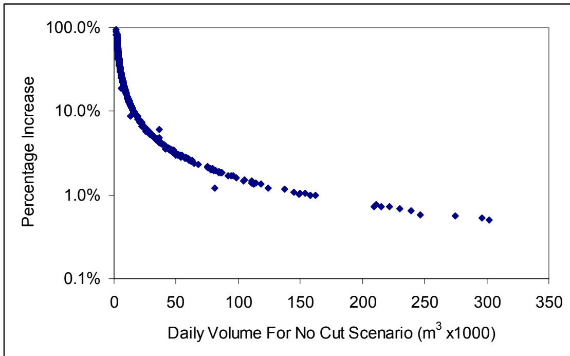
Figure 6-10. Modeled percentage change in peak discharge rate for harvested vs. un-harvested scenarios in North Fork Caspar Creek, CA.
