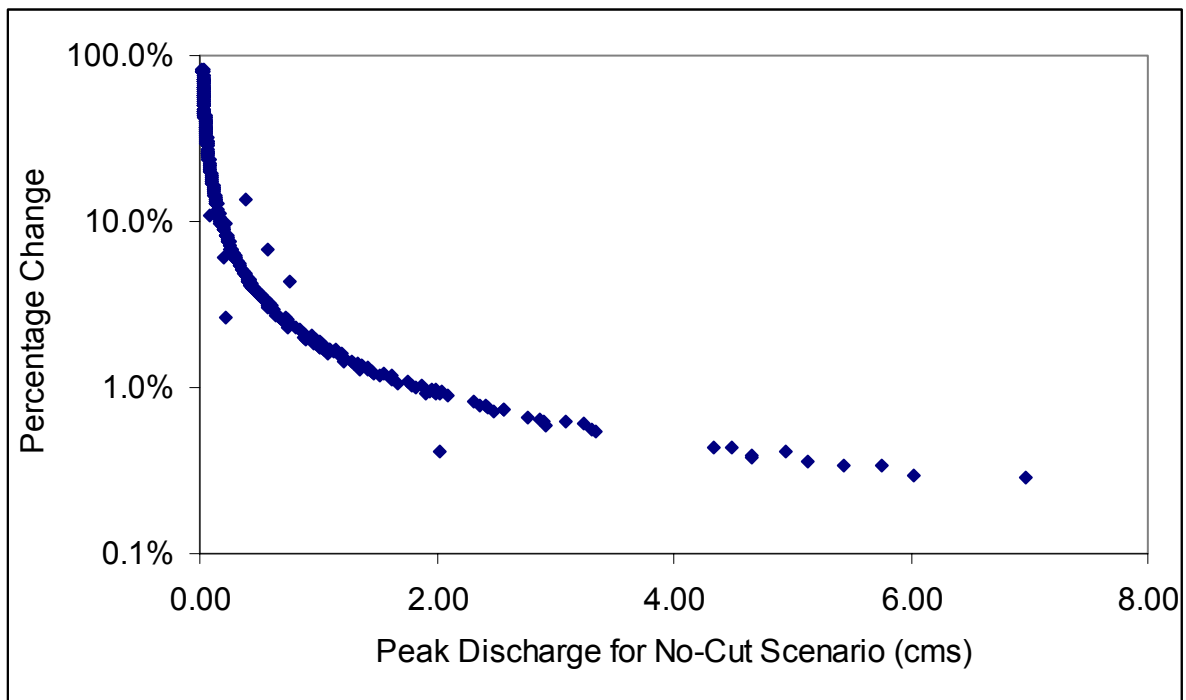
Figure 6-8. Modeled percentage change in peak discharge rate for harvested vs. un-harvested scenarios in North Fork Caspar Creek, CA.
