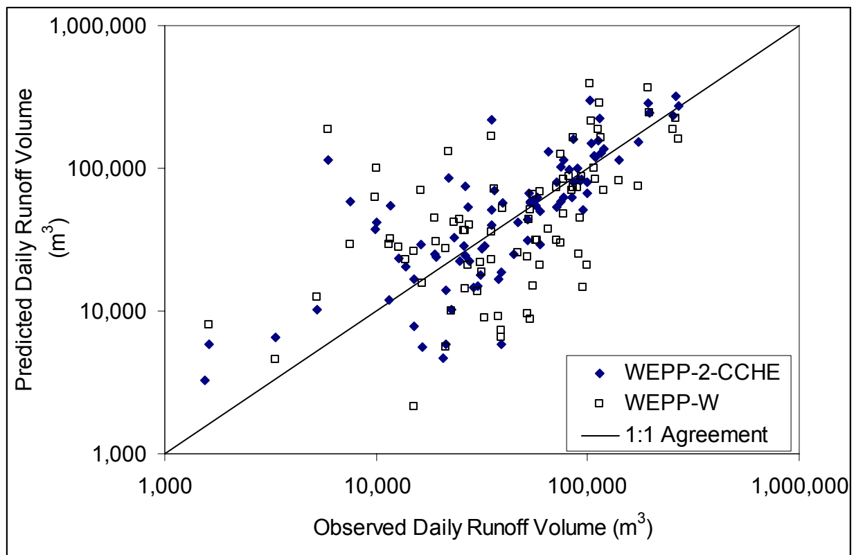
Figure 3-9. Observed vs. predicted daily runoff volume for 89 events at South Fork Caspar Creek Experimental Watershed, CA (1995-1997).
