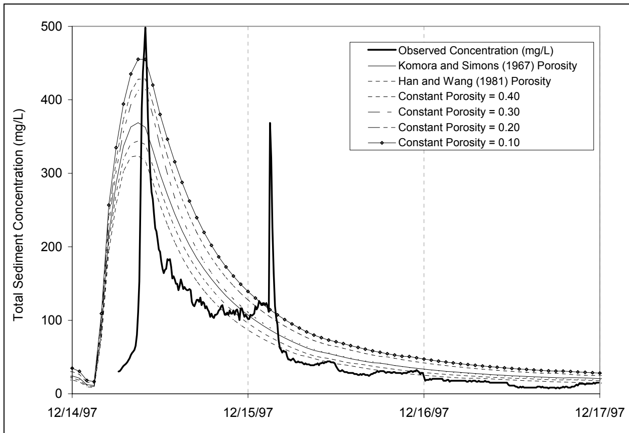
Figure 5-13. Example differences in hydrographs for changes in bed material porosity options from originally used option (Komura and Simons, 1967) for a selected runoff event in South Fork Caspar Creek, CA.
