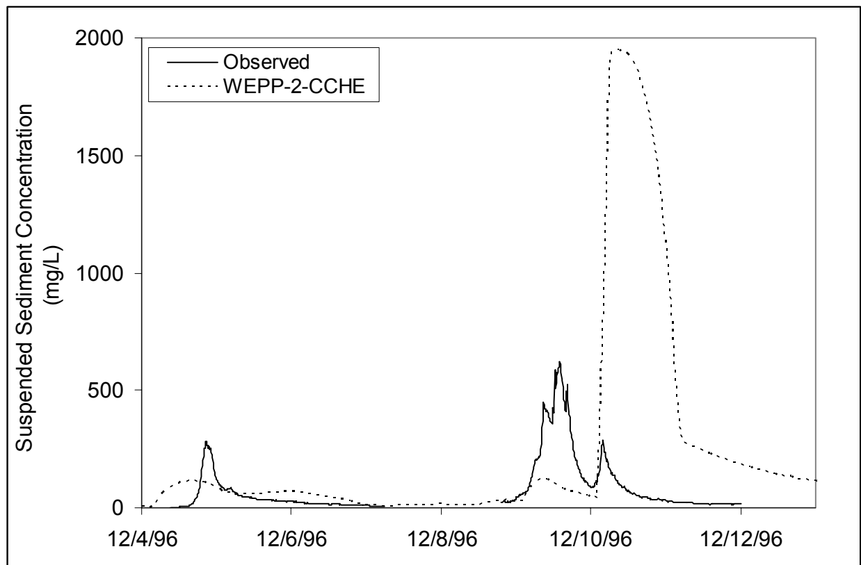
Figure 4-4. Predicted and observed hourly suspended sediment concentration for South Fork Caspar Creek simulation (04 December 1996 thru 05 January 1997).
