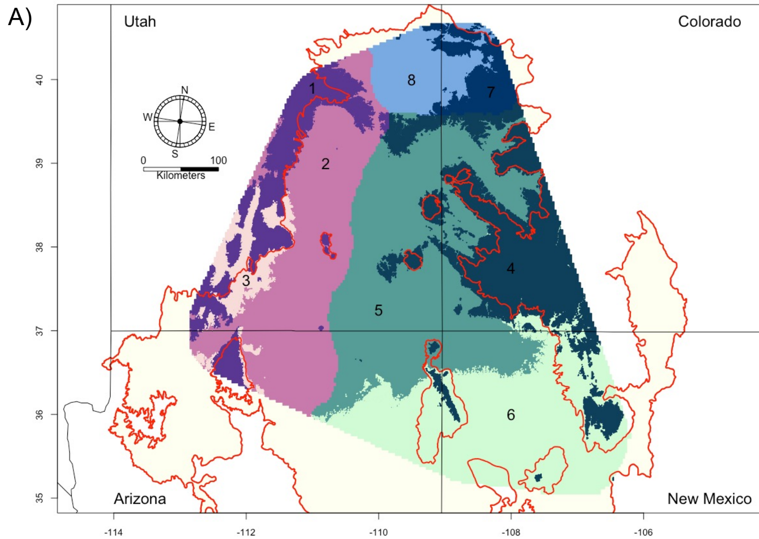
Figure 1. Seed transfer zones (A) and zone statistics for mean annual precipitation and temperature seasonality (B), the environmental variables influencing adaptation across Astragalus lonchocarpus ’ regional distribution. Numbers in (A) refer to the zones along the x-axis in (B). The red polygon in (A) represents the Colorado Plateau boundary.
