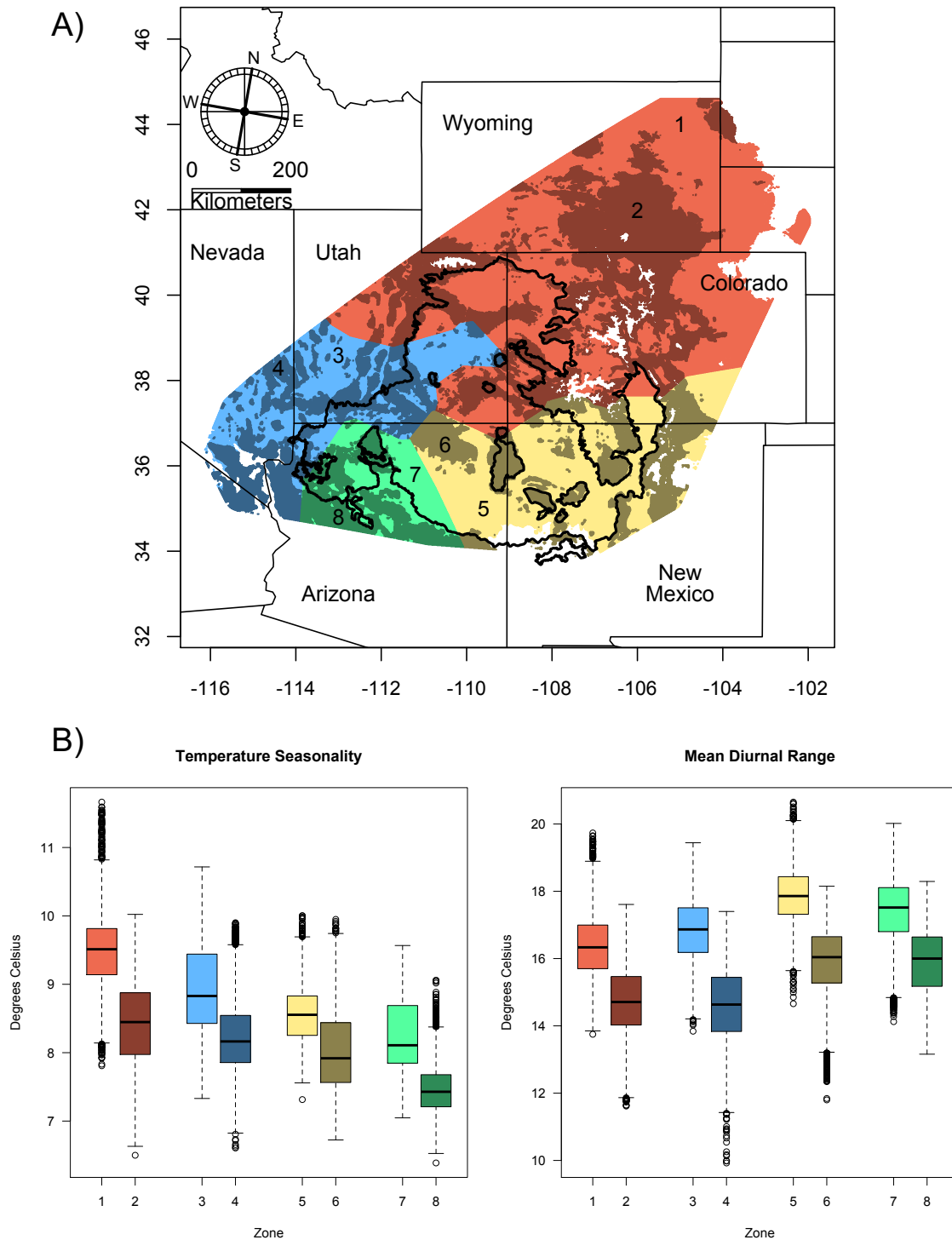
Figure 2. Seed transfer zones (A) and zone statistics for temperature seasonality and mean diurnal range (B), the environmental variables influencing adaptation across Machaeranthera canescens ' regional distribution. Numbers in (A) refer to the zones along the x-axis in (B). Uncolored areas within the seed transfer zones represent locations outside of the species' environmental tolerance. The black polygon represents the Colorado Plateau boundary.
