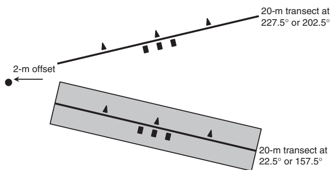
Fig. 1. Planar intersect method of sampling fuels and coarse woody debris. ● represents the grid point ( n=36 per unit, total n=432 ), ▲ represents litter and duff depth measurements (at 5, 10, 15 m), ■ represents vertical height measurements (at 8, 10, 12 m), thick lines represent two 20-m transects, shaded box represents 80 m 2 coarse woody debris belt-transect. The 1-h and 10-h fuels are tallied between 8 and 12 m on each transect. The 100-h fuels are tallied between 9 and 11 m on each transect. The 1000-h fuel species, diameter and decay status (sound or rotten) are tallied along the entire 20 m of each transect. Coarse woody debris species, large diameter (diameter > 15 cm), small diameter, length, decay class (decay class I–V [Brown 1974]) and rating (more or less than 50% of log located in transect) are measured within the belt-transect. Figure adapted from Yaussy (2001).
