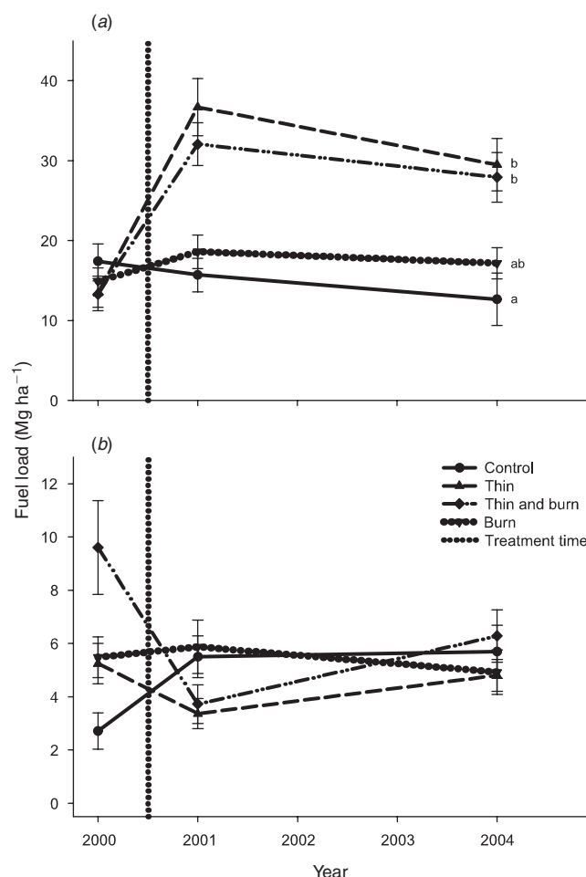
Fig. 5. Mean fuel load values for (a) 1000-h sound, and (b) 1000-h rotten fuels. Pre-treatment values are given for the 2000 data, post-treatment values are given for 2001 and 2004. Error bars represent the standard error of the mean. Statistically significant differences are represented by different letters within each graph. Note different scales on the y-axes.
