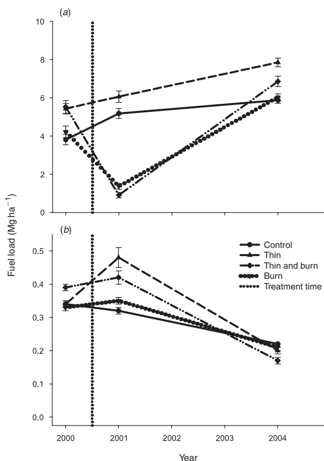
Fig. 2. Mean fuel load values for (a) litter and (b) duff. Pre-treatment values are given for 2000, post-treatment values are given for 2001 and 2004. Error bars represent the standard error of the mean. Statistically significant differences are represented by different letters within each graph. Note different scales on the y-axes.
