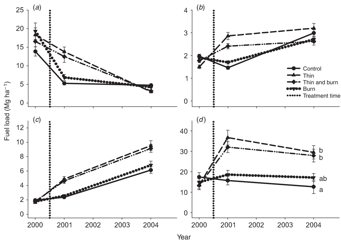
Fig. 3. Mean fuel load values for (a) 1-h fuels, (b) 10-h fuels, (c) 100-h fuels, and (d) 1000-h sound fuels. Pre-treatment values are given for the 2000 data, post-treatment values are given for 2001 and 2004. Error bars represent the standard error of the mean. Statistically significant differences are represented by different letters within each graph. Note different scales on the y-axes.
