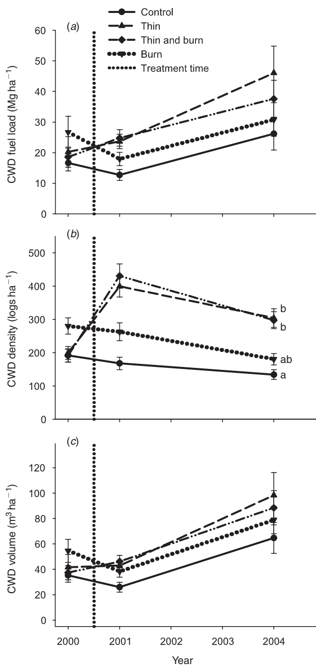
Fig. 4. Mean values for coarse woody debris (CWD) (a) mass, (b) density, and (c) volume. Pre-treatment values are given for the 2000 data, post-treatment values are given for 2001 and 2004. Error bars represent the standard error of the mean. Statistically significant differences are represented by different letters within each graph. Note different y-axes.
